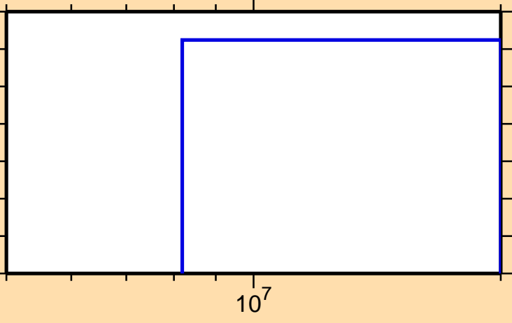
\sigma vs. E for ^{143}\text{Nd}(n,np)
