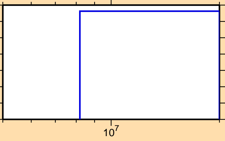
\sigma vs. E for ^{143}\text{Nd}(n,p\alpha)
