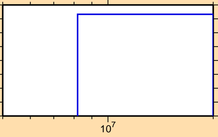
\sigma vs. E for ^{143}\text{Nd}(n,2np)
