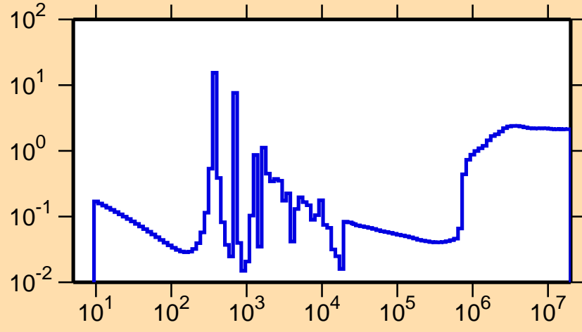
\sigma vs. E for ^{144}\text{Nd}(n,\text{nonel.})
