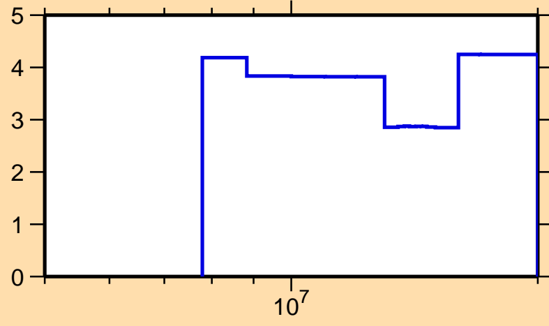
\Delta\sigma/\sigma vs. E for ^{144}\text{Nd}(n,2n)
