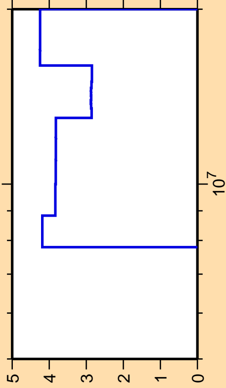
\Delta\sigma/\sigma vs. E for ^{144}\text{Nd}(n,2n)
