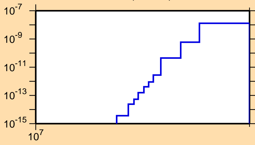
\sigma vs. E for ^{144}\text{Nd}(n,\text{He3})
