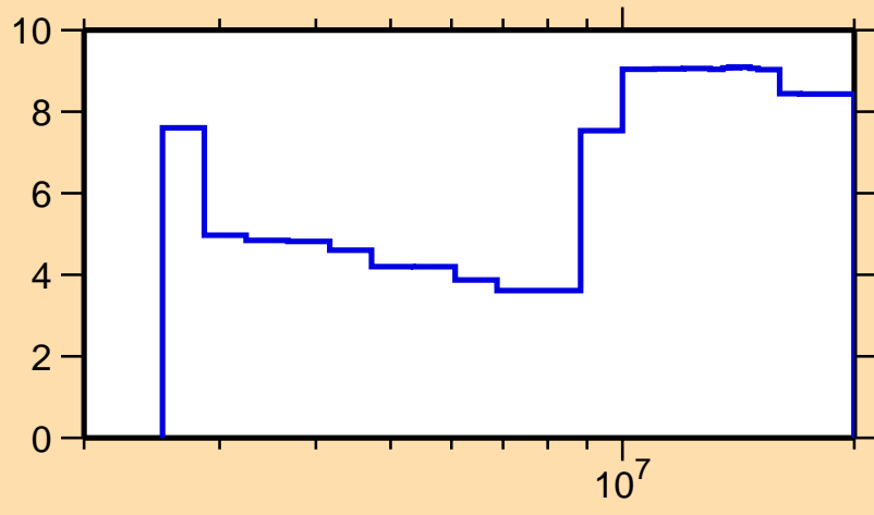
\Delta\sigma/\sigma vs. E for ^{144}\text{Nd}(n,n\text{cont.})
