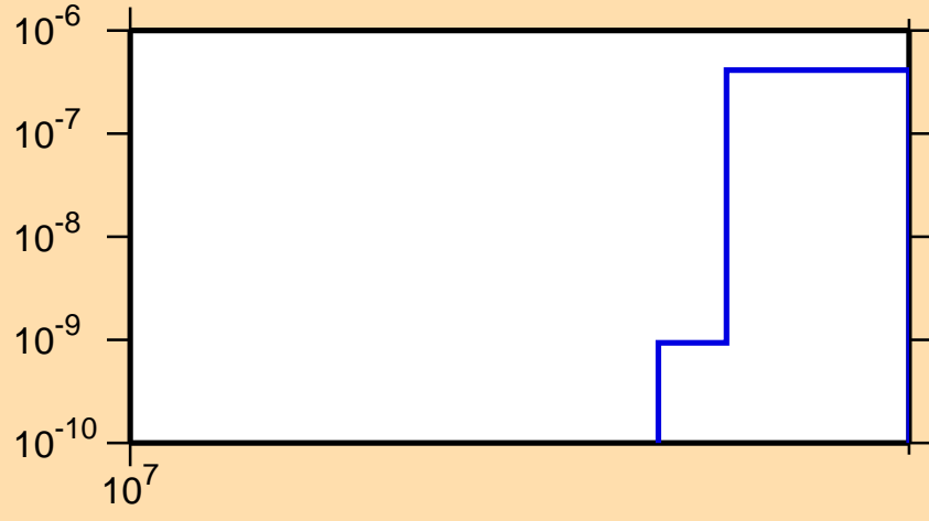
\sigma vs. E for ^{144}\text{Nd}(n,nt)
