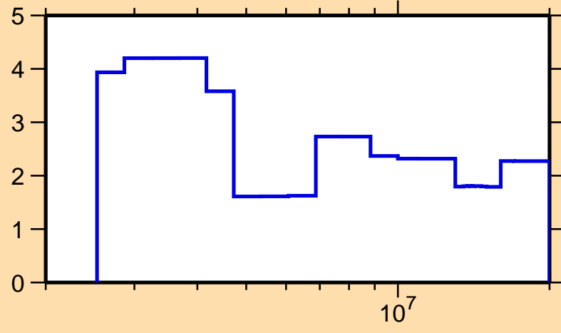
\Delta\sigma/\sigma vs. E for ^{144}\text{Nd}(n, el.)
