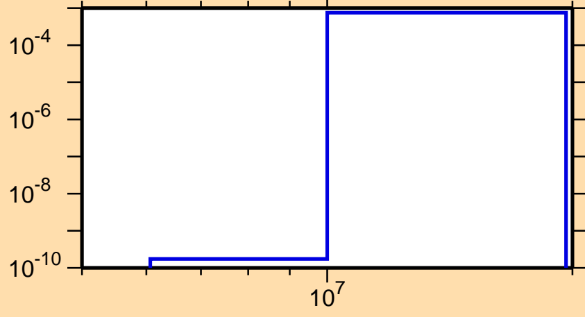
\sigma vs. E for ^{144}\text{Nd}(n,d)
