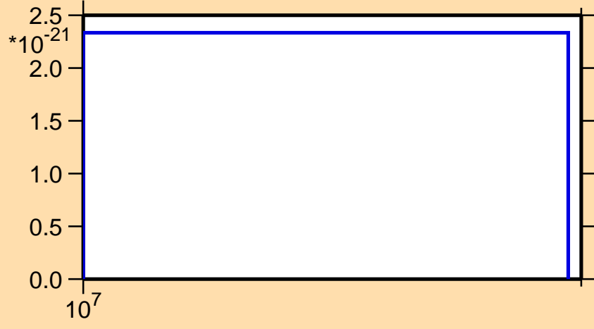
\sigma vs. E for ^{144}\text{Nd}(\text{mt } 11)
