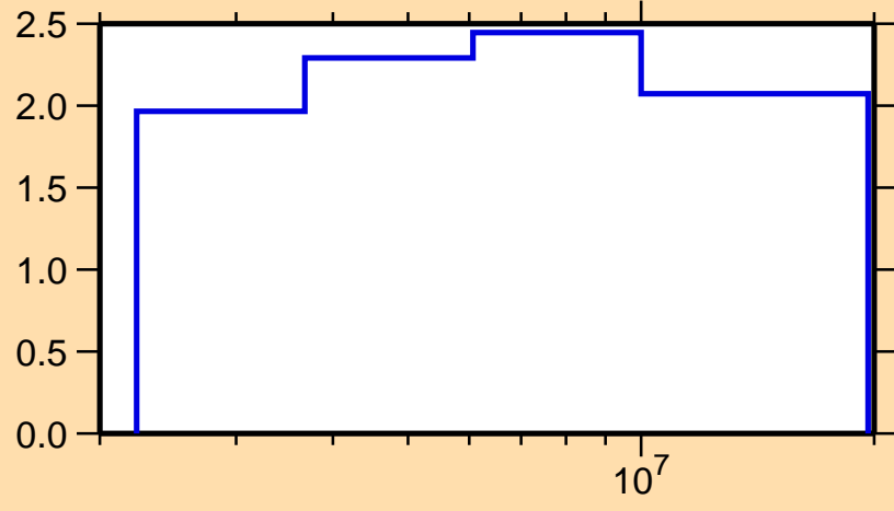
\Delta\sigma/\sigma vs. E for ^{144}\text{Nd}(n,n\text{onel.})
