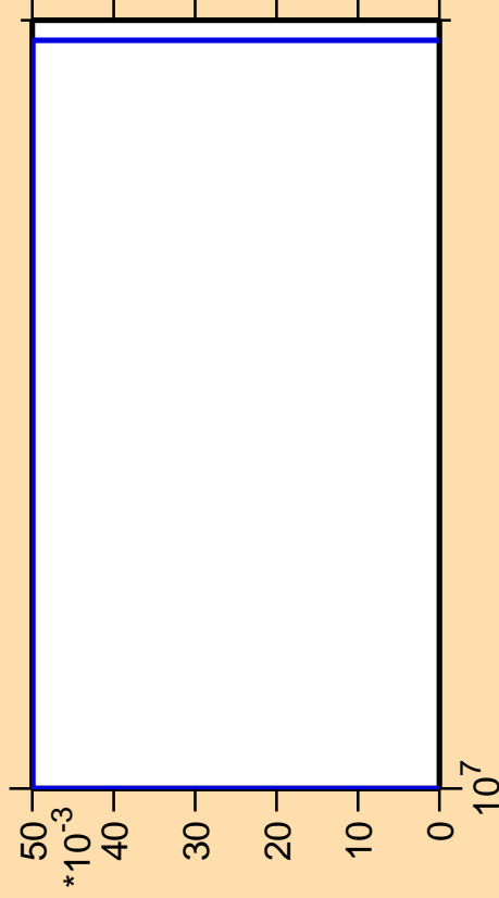
\Delta\sigma/\sigma vs. E for ^{144}\text{Nd}(\text{mt } 45)
