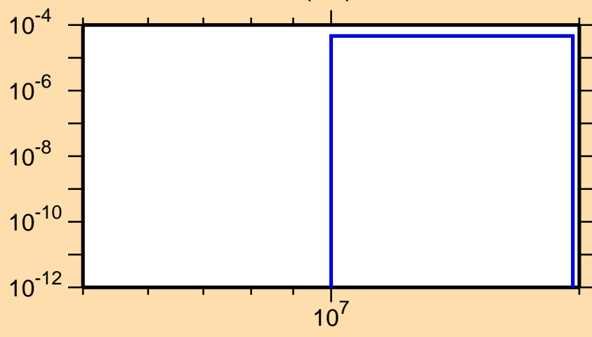
\sigma vs. E for ^{144}\text{Nd}(n,t)
