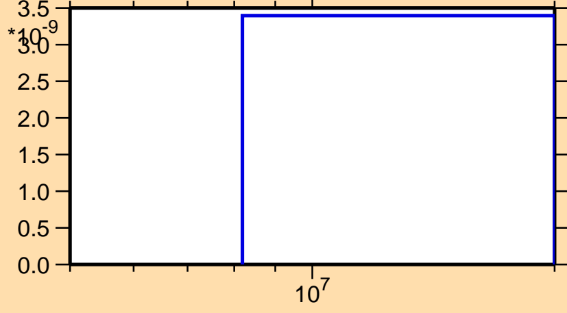
\sigma vs. E for ^{144}\text{Nd}(n,nt)
