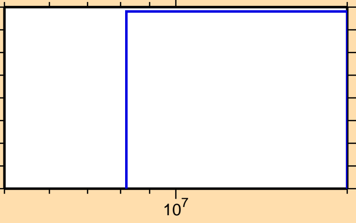
\sigma vs. E for ^{144}\text{Nd}(n,p\alpha)
