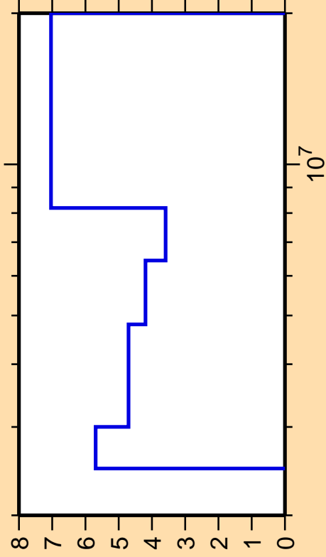
\Delta\sigma/\sigma vs. E for ^{144}\text{Nd}(n,n\text{cont.})
