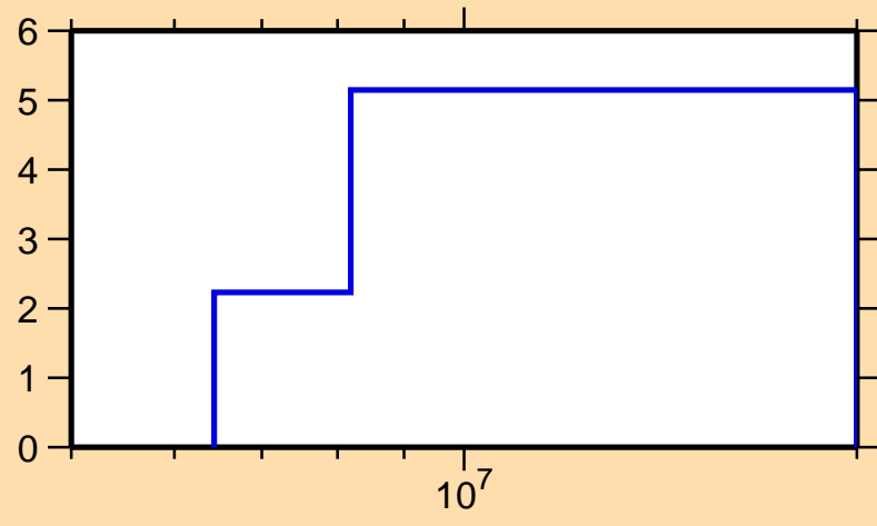
\Delta\sigma/\sigma vs. E for ^{144}\text{Nd}(n,\text{inel.})
