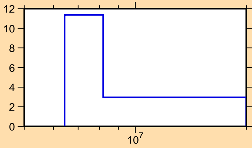
\Delta\sigma/\sigma vs. E for ^{144}\text{Nd}(n,2n)
