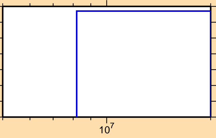
\sigma vs. E for ^{144}\text{Nd}(n,\text{He}3)
