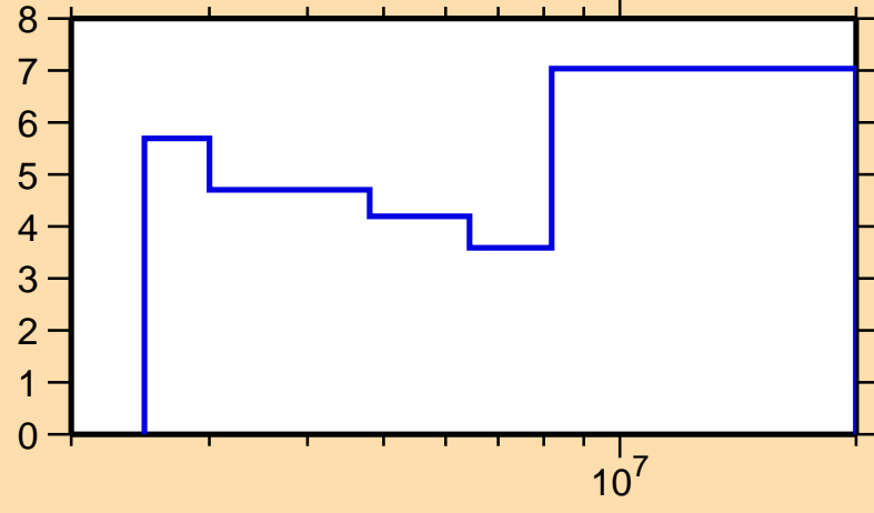
\Delta\sigma/\sigma vs. E for ^{144}\text{Nd}(n,n\text{cont.})
