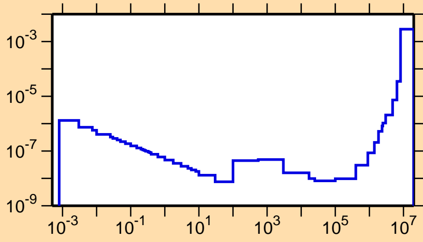
\sigma vs. E for ^{144}\text{Nd}(n,\alpha)
