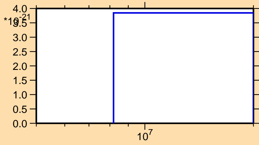
\sigma vs. E for ^{144}\text{Nd}(\text{mt } 11)
