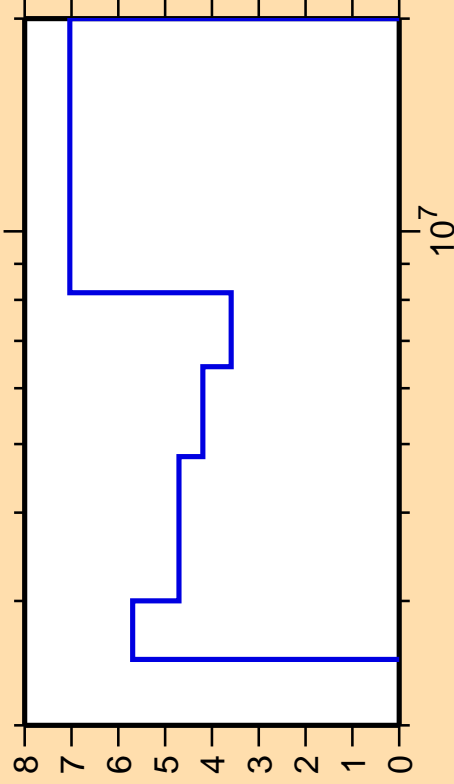
\Delta\sigma/\sigma vs. E for ^{144}\text{Nd}(n,n\text{cont.})
