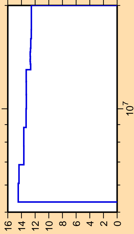
\Delta\sigma/\sigma vs. E for ^{145}\text{Nd}(n,n_1)
