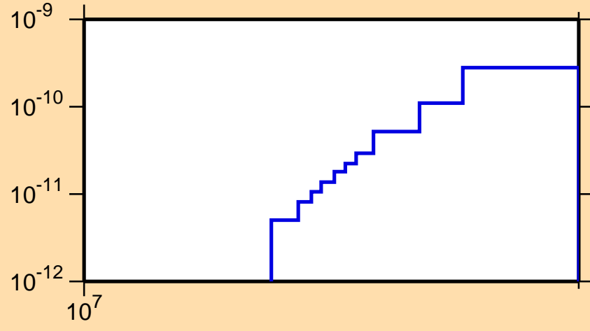
\sigma vs. E for ^{145}\text{Nd}(n,p\alpha)
