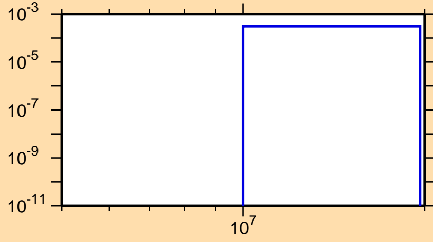
\sigma vs. E for ^{145}\text{Nd}(n,np)
