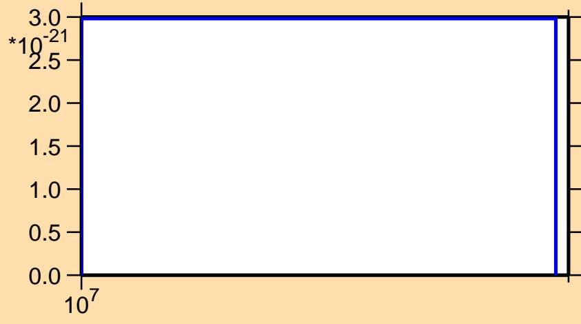
\sigma vs. E for ^{145}\text{Nd} (mt 11)
