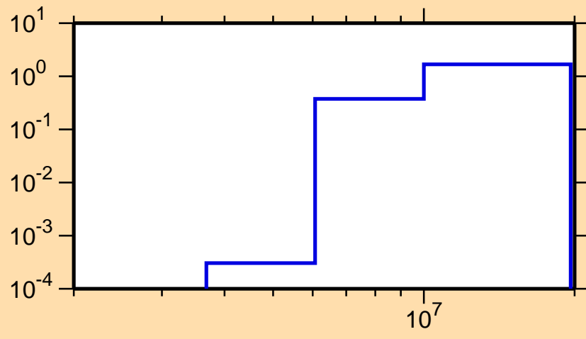
\sigma vs. E for ^{145}\text{Nd}(n,2n)
