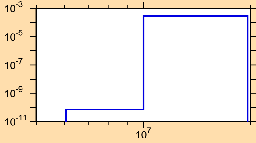
\sigma vs. E for ^{145}\text{Nd}(n,t)
