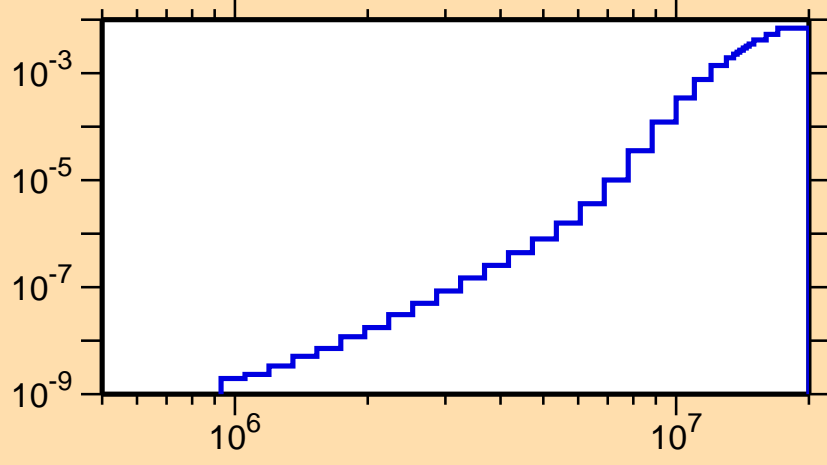
\sigma vs. E for ^{146}\text{Nd}(n,\alpha)
