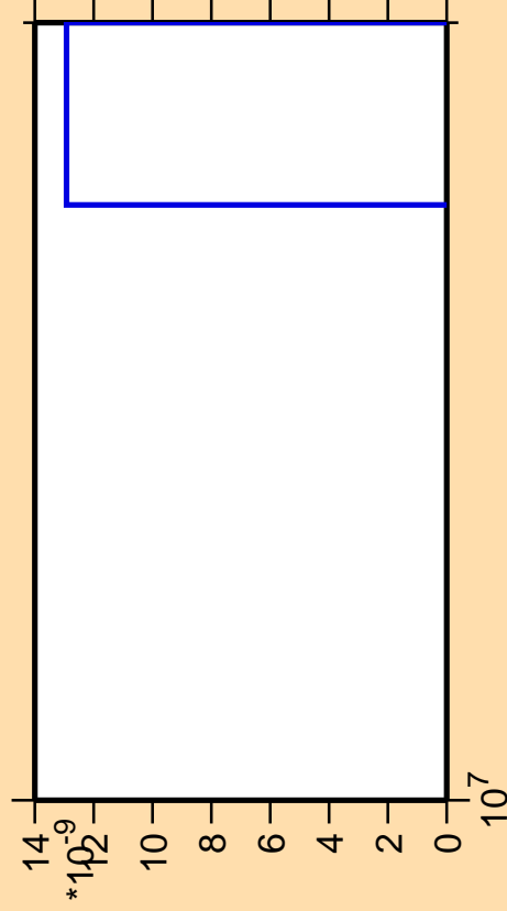
\Delta\sigma/\sigma vs. E for ^{146}\text{Nd} (mt 11)
