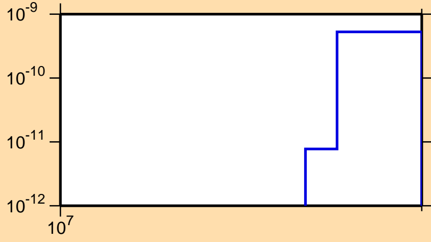
\sigma vs. E for ^{146}\text{Nd}(n,\text{He3})
