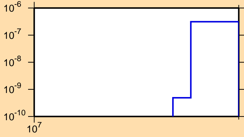
\sigma vs. E for ^{146}\text{Nd}(n,nt)
