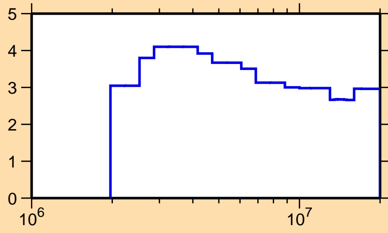
\Delta\sigma/\sigma vs. E for ^{146}\text{Nd}(n,n\text{onel.})
