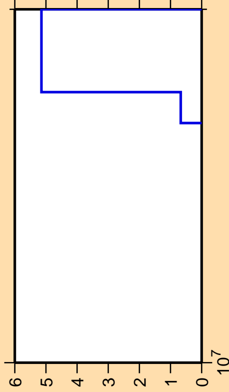
\Delta\sigma/\sigma vs. E for ^{146}\text{Nd}(n,p\alpha)
