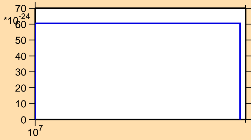
\sigma vs. E for ^{146}\text{Nd} (mt 11)
