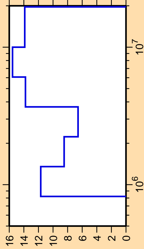
\Delta\sigma/\sigma vs. E for ^{146}\text{Nd}(n,n_4)
