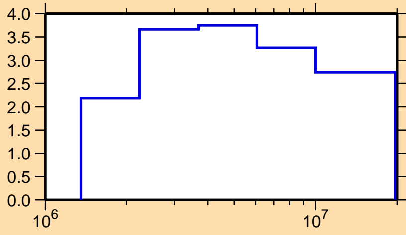
\Delta\sigma/\sigma vs. E for ^{146}\text{Nd}(n,n_{\text{nonel}})
