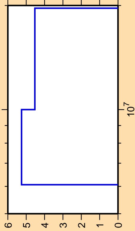
\Delta\sigma/\sigma vs. E for ^{146}\text{Nd}(n,2n)
