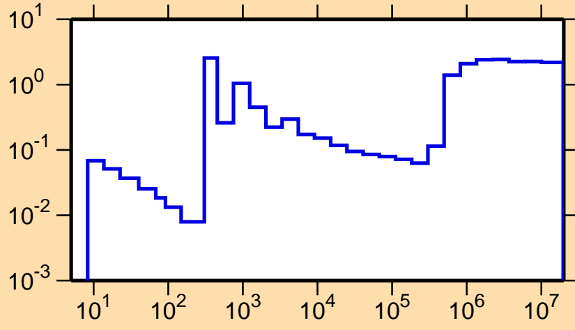
\sigma vs. E for ^{146}\text{Nd}(n,\text{nonel.})
