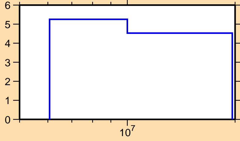
\Delta\sigma/\sigma vs. E for ^{146}\text{Nd}(n,2n)
