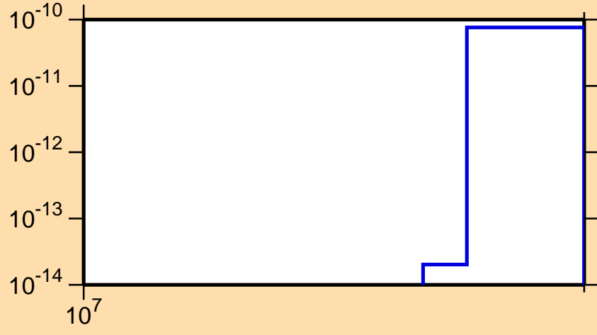
\sigma vs. E for ^{147}\text{Nd}(n,3n\alpha)
