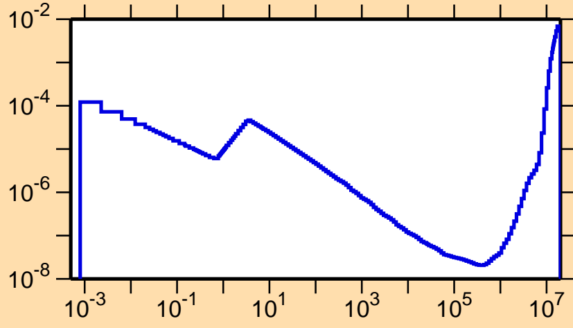
\sigma vs. E for ^{147}\text{Nd}(n,\alpha)
