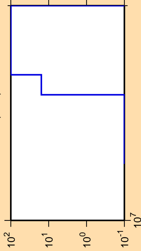
\Delta\sigma/\sigma vs. E for ^{147}\text{Nd}(n,\text{nt})
