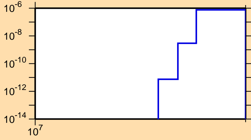
\sigma vs. E for ^{147}\text{Nd}(n,\text{nt})
