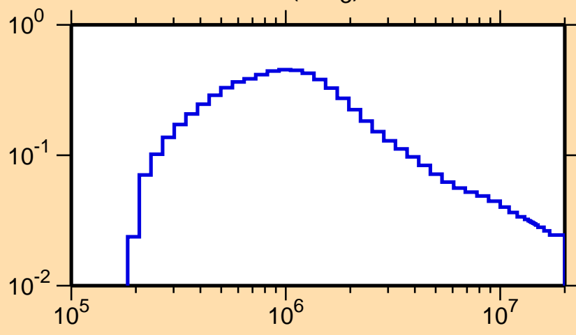
\sigma vs. E for ^{147}\text{Nd}(n,n_3)
