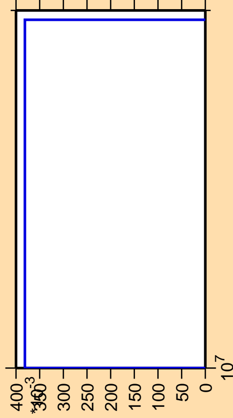
\Delta\sigma/\sigma vs. E for ^{147}\text{Nd}(n,p\alpha)
