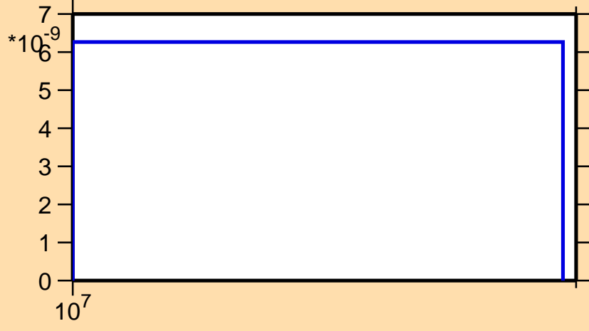
\sigma vs. E for ^{147}\text{Nd}(n,nt)
