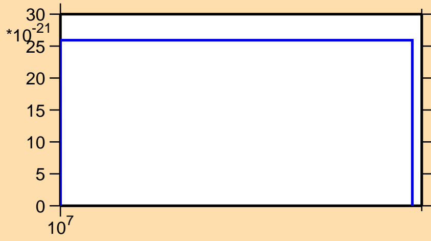
\sigma vs. E for ^{147}\text{Nd} (mt 11)
