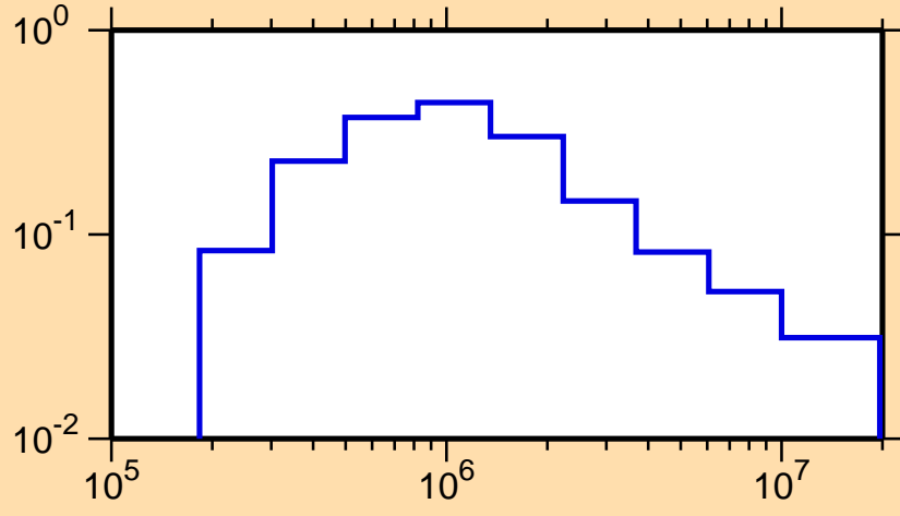
\sigma vs. E for ^{147}\text{Nd}(n,n_3)
