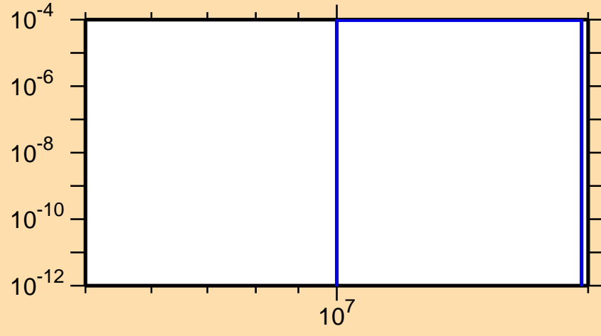
\sigma vs. E for ^{147}\text{Nd}(n,np)
