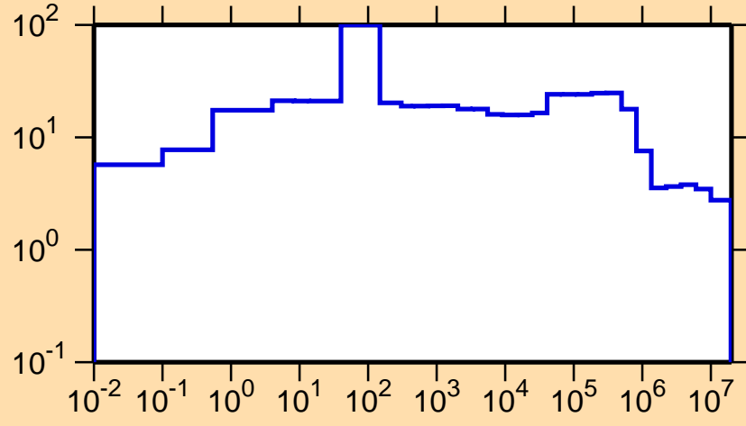
\Delta\sigma/\sigma vs. E for ^{147}\text{Nd}(n,\text{nonel.})
