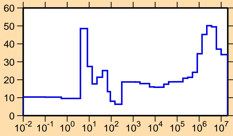
\Delta\sigma/\sigma vs. E for ^{147}\text{Nd}(n,\gamma)
