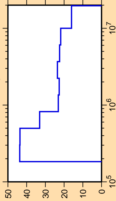
\Delta\sigma/\sigma vs. E for ^{147}\text{Nd}(n,n_3)
