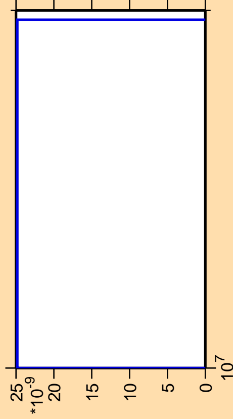
\Delta\sigma/\sigma vs. E for ^{147}\text{Nd} (mt 11)
