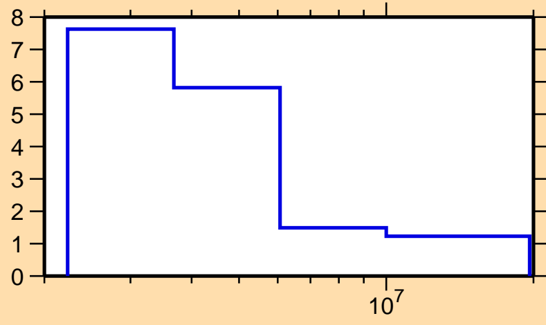
\Delta\sigma/\sigma vs. E for ^{147}\text{Nd}(n,\text{el.})
