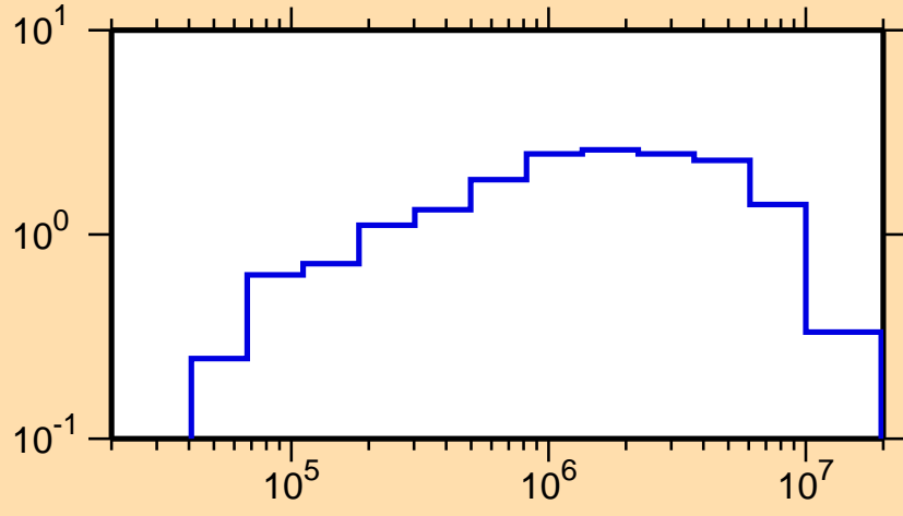
\sigma vs. E for ^{147}\text{Nd}(n,\text{inel.})
