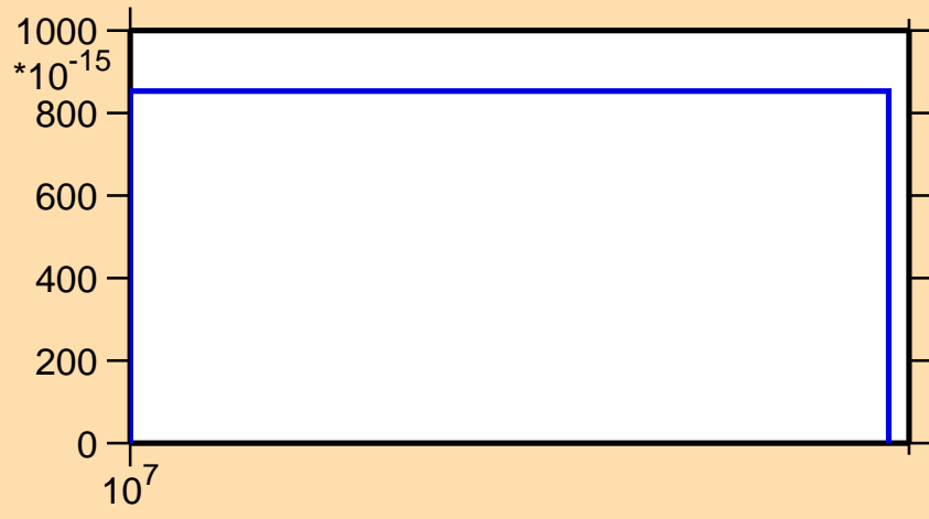
\sigma vs. E for ^{147}\text{Nd}(n,\text{He}3)
