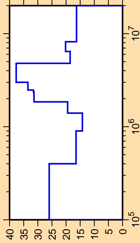
\Delta\sigma/\sigma vs. E for ^{147}\text{Nd}(n,n_4)
