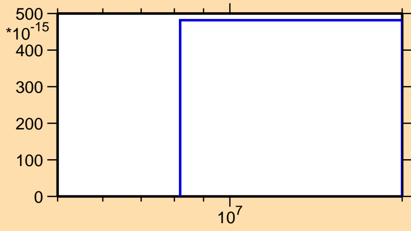
\sigma vs. E for ^{147}\text{Nd}(n,p\alpha)
