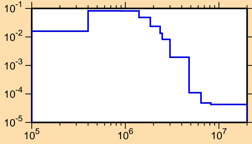
\sigma vs. E for ^{147}\text{Nd}(n,n_4)
