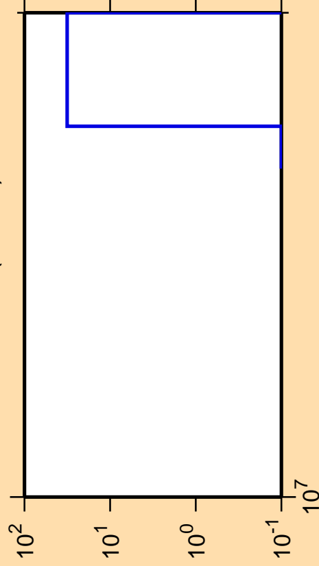
\Delta\sigma/\sigma vs. E for ^{148}\text{Nd}(n,\text{He}3)
