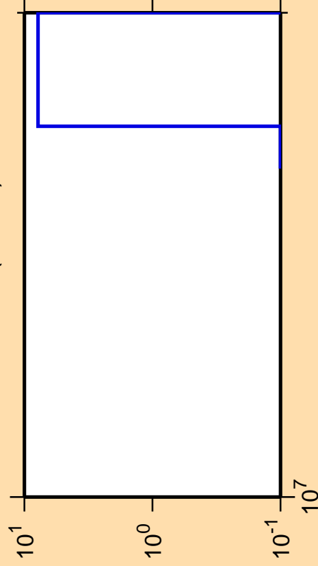
\Delta\sigma/\sigma vs. E for ^{148}\text{Nd}(n,3n\alpha)
