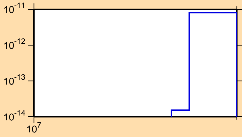
\sigma vs. E for ^{148}\text{Nd}(n,\text{He}3)
