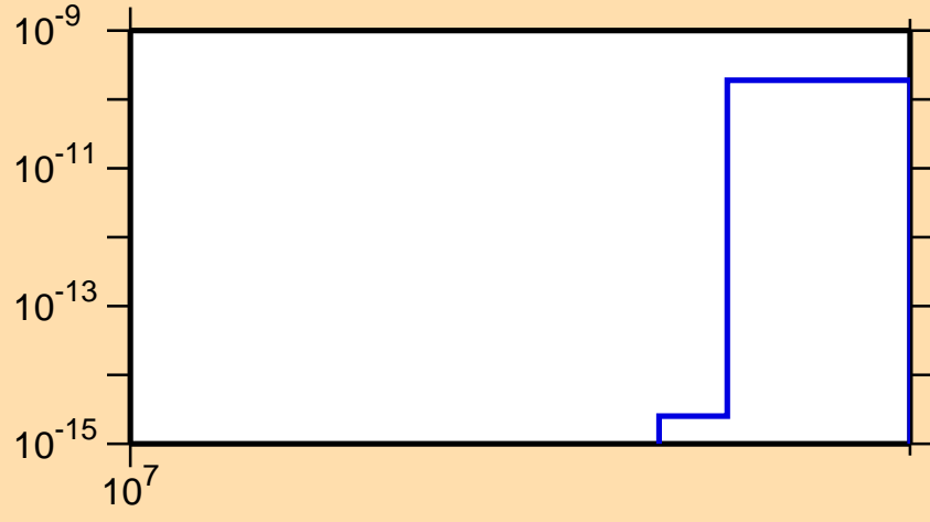
\sigma vs. E for ^{148}\text{Nd}(n,2np)
