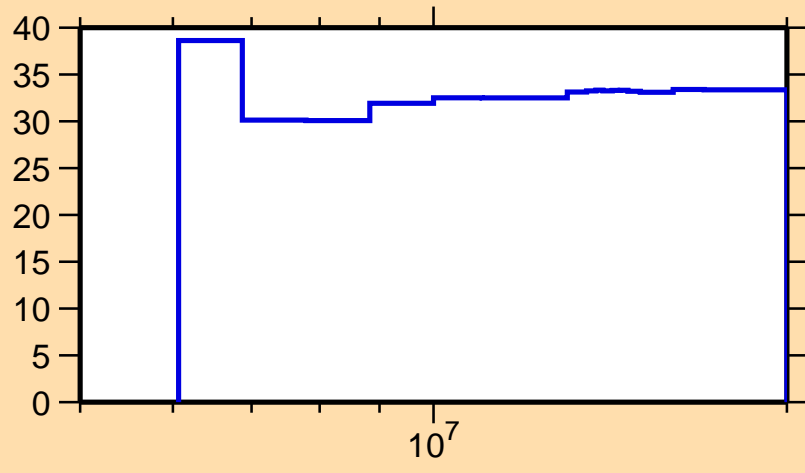
\Delta\sigma/\sigma vs. E for ^{148}\text{Nd}(n,\gamma)
