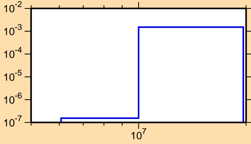
\sigma vs. E for ^{148}\text{Nd}(n,p)
