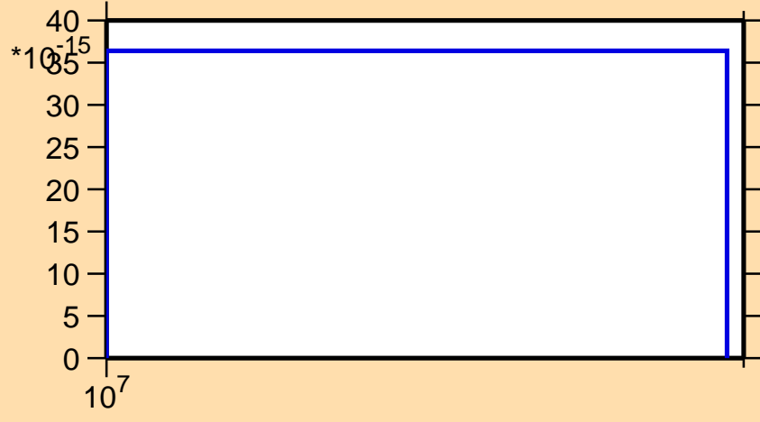
\sigma vs. E for ^{148}\text{Nd}(n,3n\alpha)
