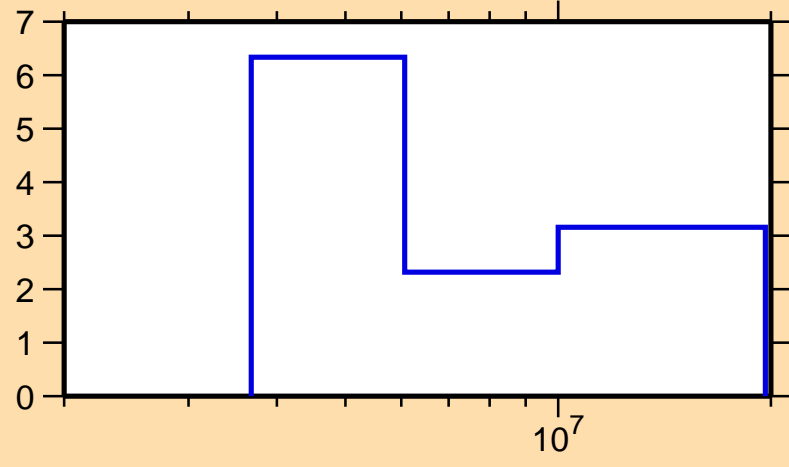
\Delta\sigma/\sigma vs. E for ^{149}\text{Nd}(n,\text{el.})
