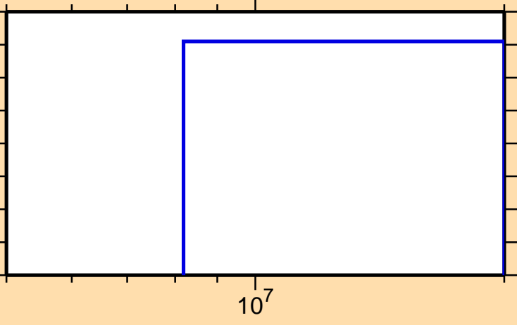
\sigma vs. E for ^{149}\text{Nd}(n,t)
