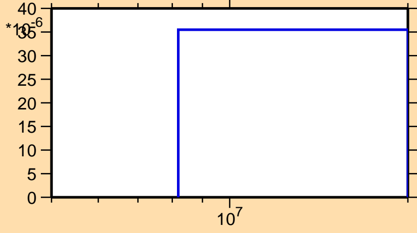
\sigma vs. E for ^{149}\text{Nd}(n,t)
