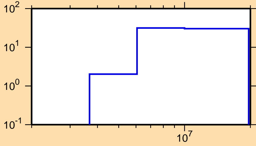
\Delta\sigma/\sigma vs. E for ^{151}\text{Nd}(n,p)
