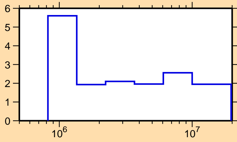
\Delta\sigma/\sigma vs. E for ^{151}\text{Nd}(n,n\text{nonel.})
