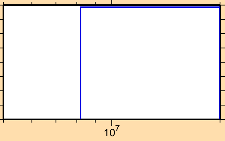
\sigma vs. E for ^{151}\text{Nd}(n,np)
