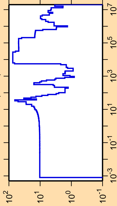
\Delta\sigma/\sigma vs. E for ^{152}\text{Nd}(n,\text{el.})
