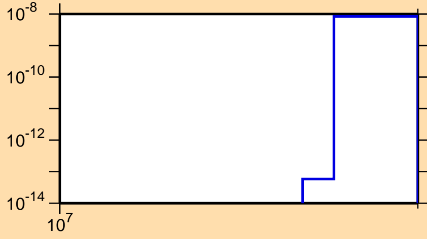
\sigma vs. E for ^{152}\text{Nd}(n,nt)
