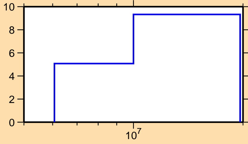
\Delta\sigma/\sigma vs. E for ^{152}\text{Nd}(n,2n)
