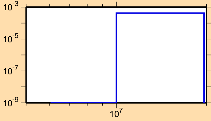
\sigma vs. E for ^{152}\text{Nd}(n,p)
