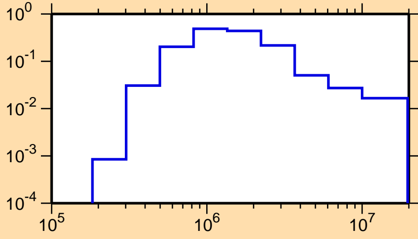
\sigma vs. E for ^{152}\text{Nd}(n,n_2)
