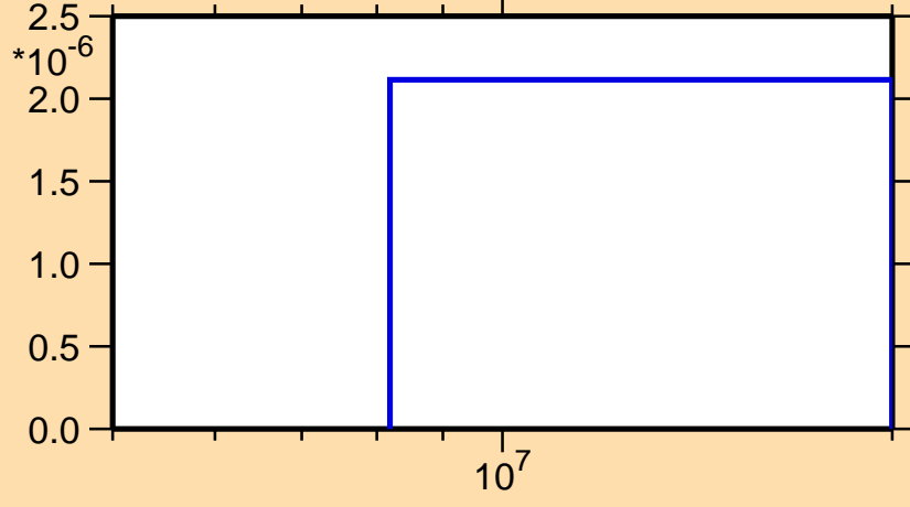
\sigma vs. E for ^{152}\text{Nd}(n,n\alpha)
