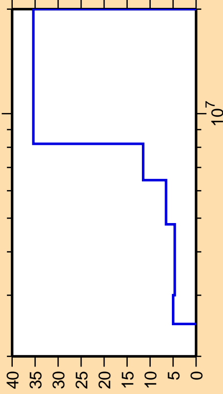
\Delta\sigma/\sigma vs. E for ^{152}\text{Nd}(n,n\text{cont.})
