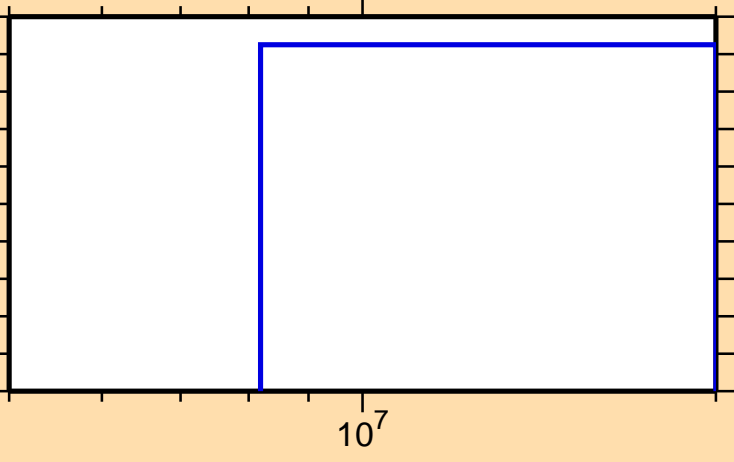
\sigma vs. E for ^{152}\text{Nd}(n,t)
