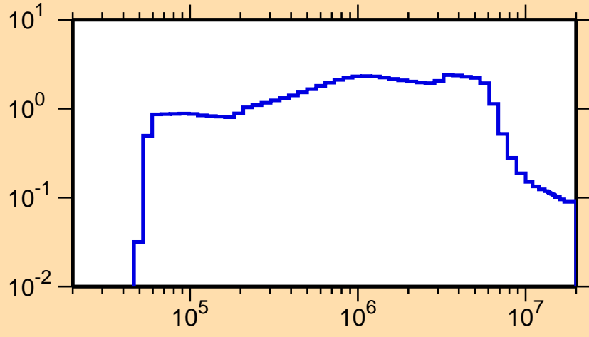
\sigma vs. E for ^{153}\text{Nd}(n,\text{inel.})
