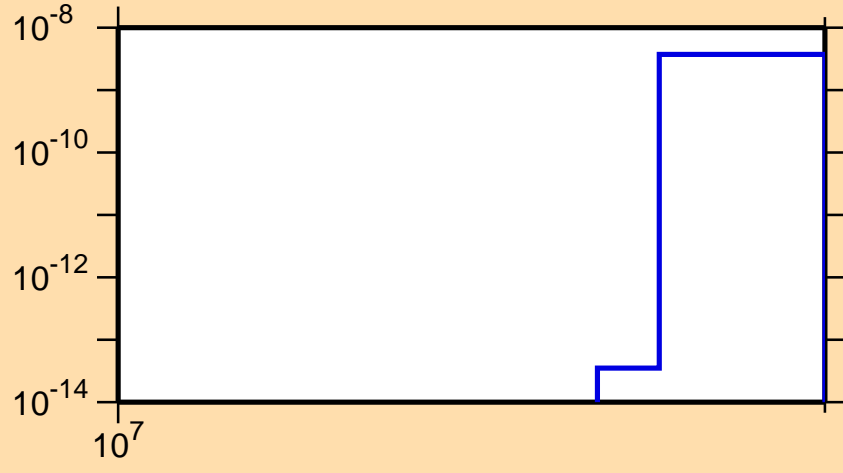
\sigma vs. E for ^{153}\text{Nd}(n,nt)
