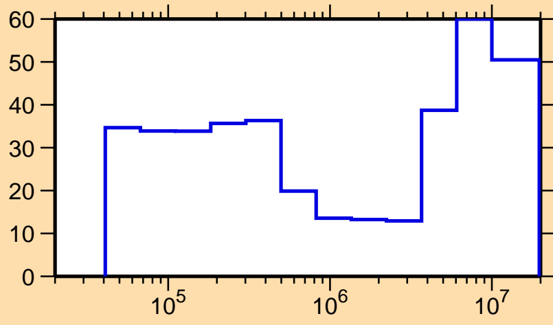
\Delta\sigma/\sigma vs. E for ^{153}\text{Nd}(n,n_1)
