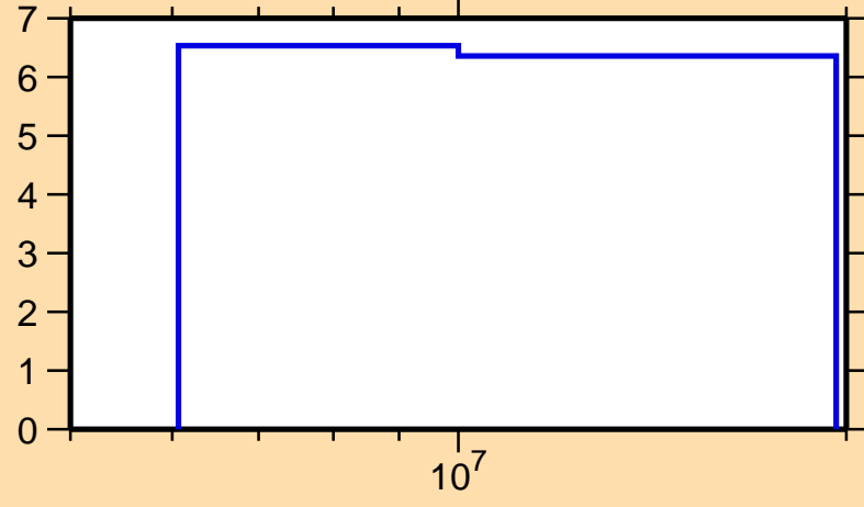
\Delta\sigma/\sigma vs. E for ^{153}\text{Nd}(n,\text{el.})
