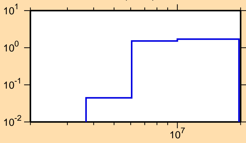
\sigma vs. E for ^{153}\text{Nd}(n,2n)
