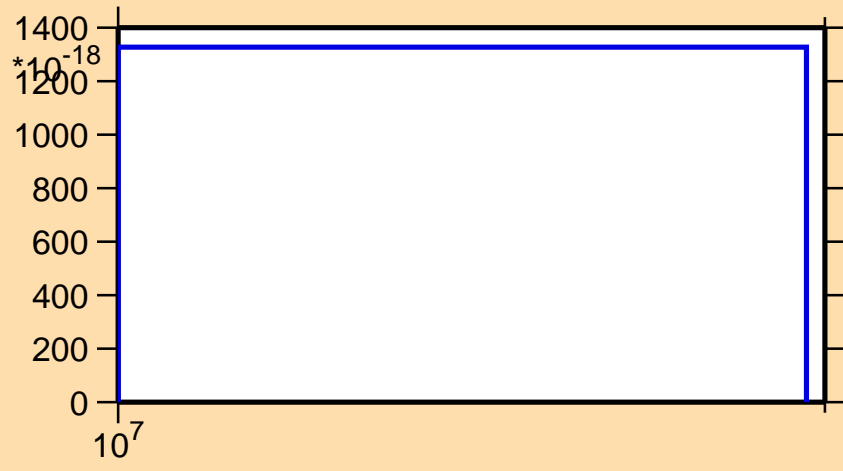
\sigma vs. E for ^{154}\text{Nd}(n,2np)
