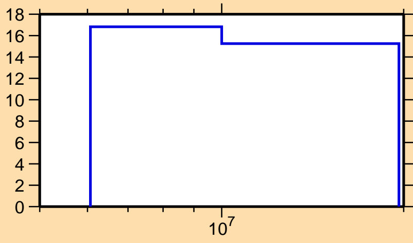
\Delta\sigma/\sigma vs. E for ^{154}\text{Nd}(n,n\text{cont.})
