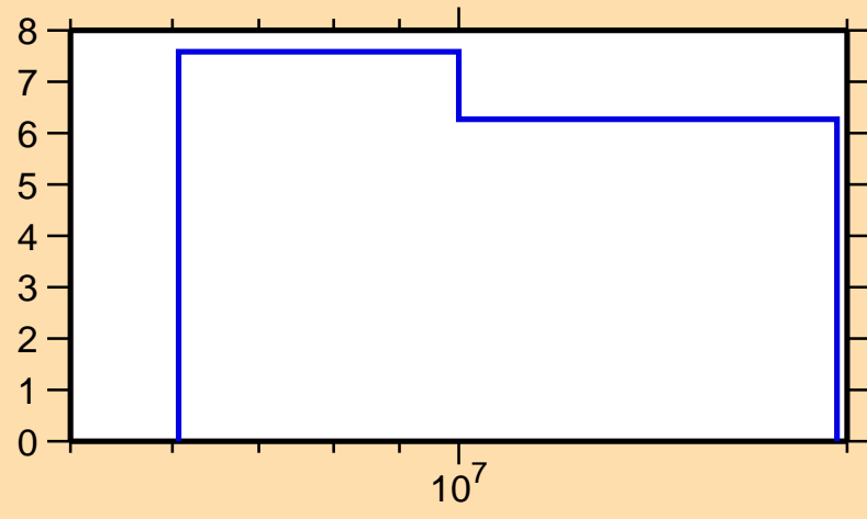
\Delta\sigma/\sigma vs. E for ^{154}\text{Nd}(n,\text{nonel.})
