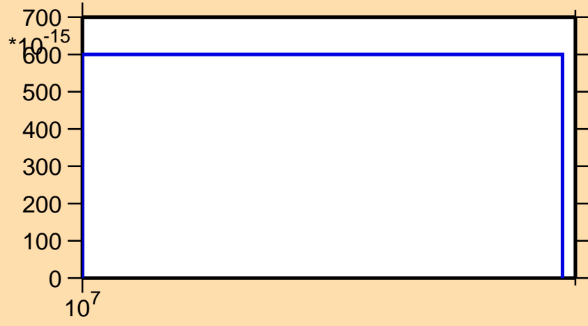
\sigma vs. E for ^{154}\text{Nd}(n,2n\alpha)
