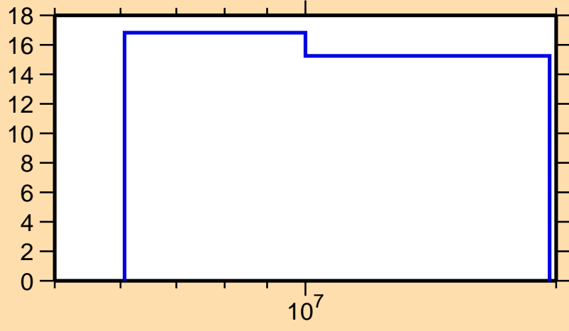
\Delta\sigma/\sigma vs. E for ^{154}\text{Nd}(n,ncont.)
