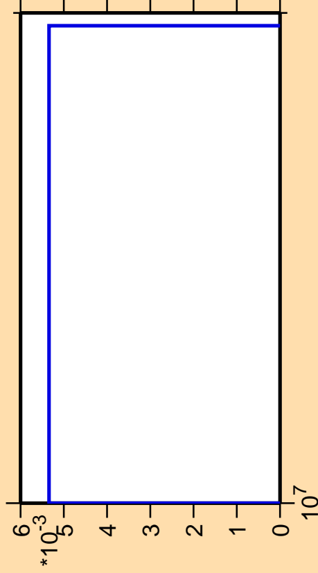
\Delta\sigma/\sigma vs. E for ^{154}\text{Nd}(n,2np)
