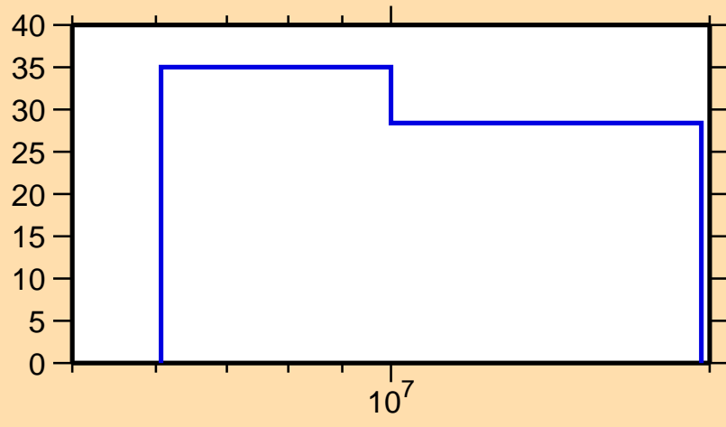
\Delta\sigma/\sigma vs. E for ^{154}\text{Nd}(n,n_1)
