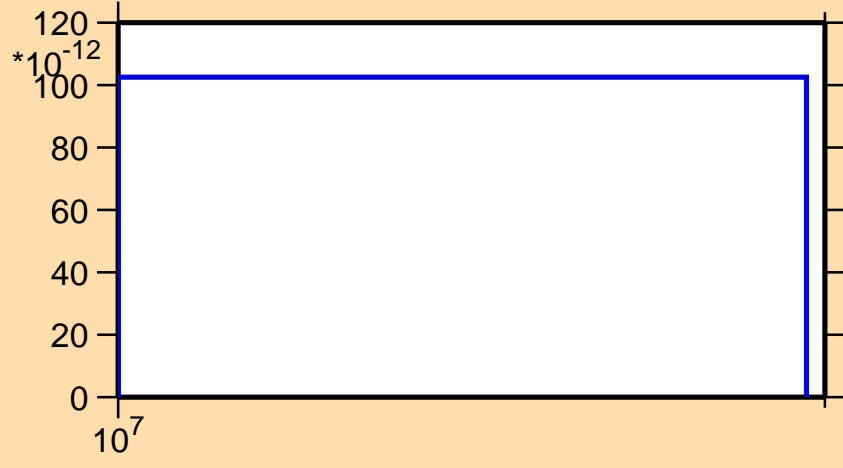
\sigma vs. E for ^{154}\text{Nd}(n,nt)
