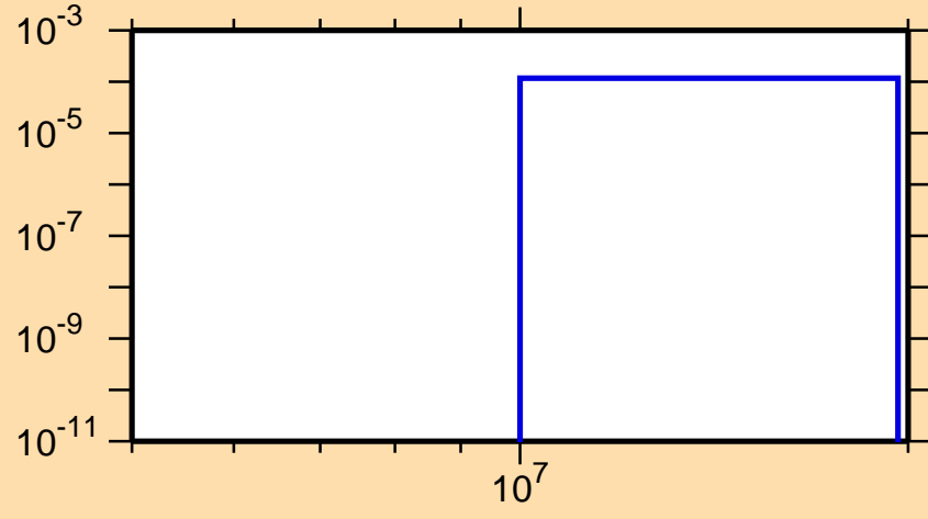
\sigma vs. E for ^{154}\text{Nd}(n,p)
