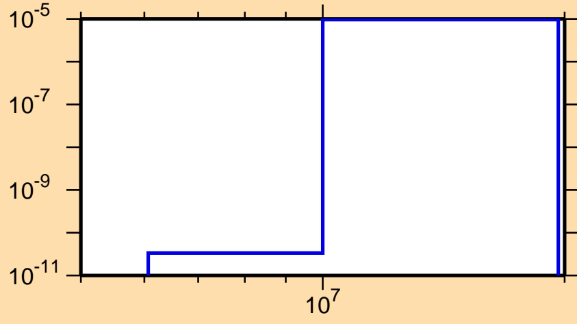
\sigma vs. E for ^{154}\text{Nd}(n,\alpha)
