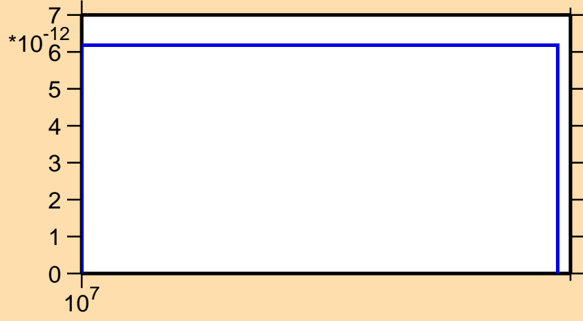
\sigma vs. E for ^{154}\text{Nd}(n,\text{nd})
