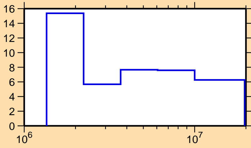
\Delta\sigma/\sigma vs. E for ^{154}\text{Nd}(n,\text{nonel.})
