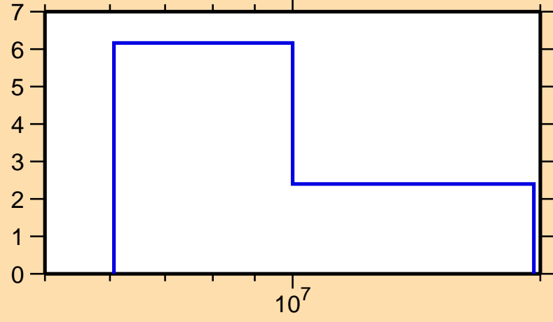
\Delta\sigma/\sigma vs. E for ^{154}\text{Nd}(n,\text{tot.})
