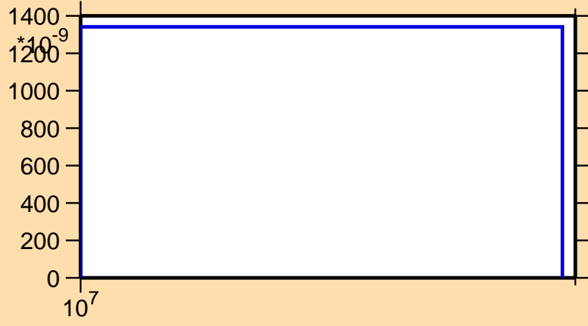
\sigma vs. E for ^{154}\text{Nd}(n,np)
