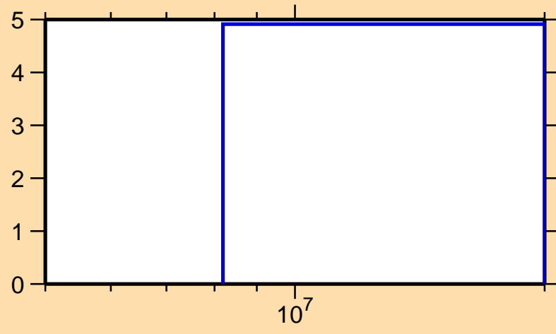
\Delta\sigma/\sigma vs. E for ^{154}\text{Nd}(n,\text{el.})
