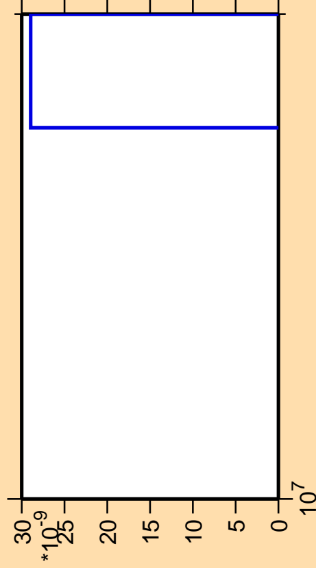
\Delta\sigma/\sigma vs. E for ^{155}\text{Nd} (mt 11)
