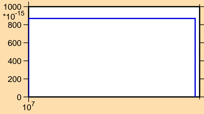
\sigma vs. E for ^{155}\text{Nd}(n,2np)
