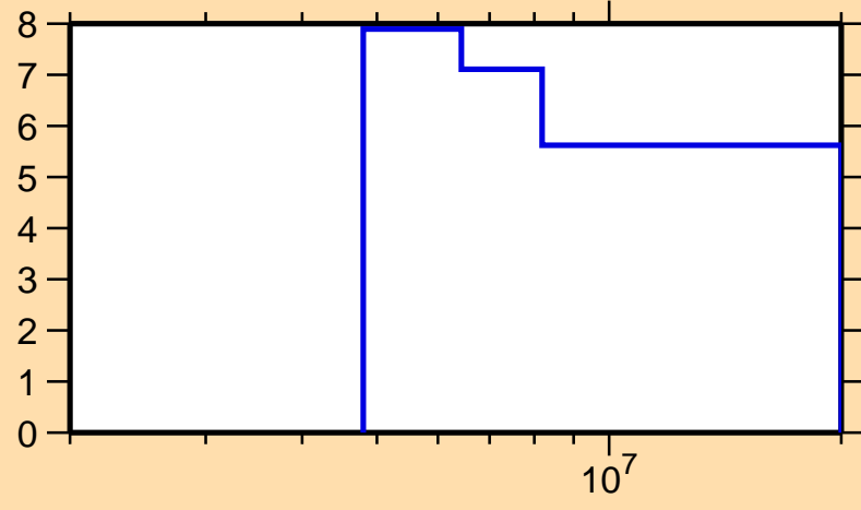
\Delta\sigma/\sigma vs. E for ^{155}\text{Nd}(n,\text{nonel.})
