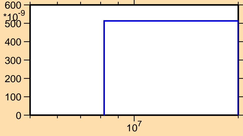
\sigma vs. E for ^{155}\text{Nd}(n,np)
