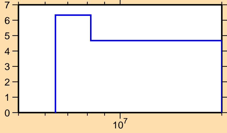
\Delta\sigma/\sigma vs. E for ^{155}\text{Nd}(n,\text{tot.})
