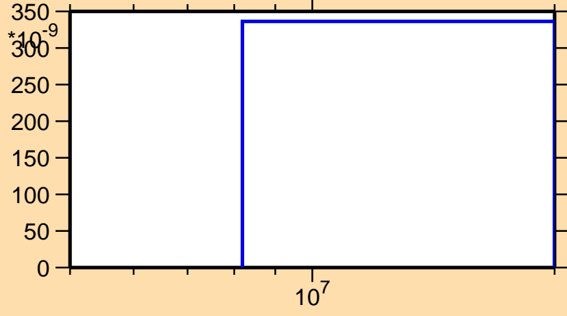
\sigma vs. E for ^{155}\text{Nd}(n,n\alpha)
