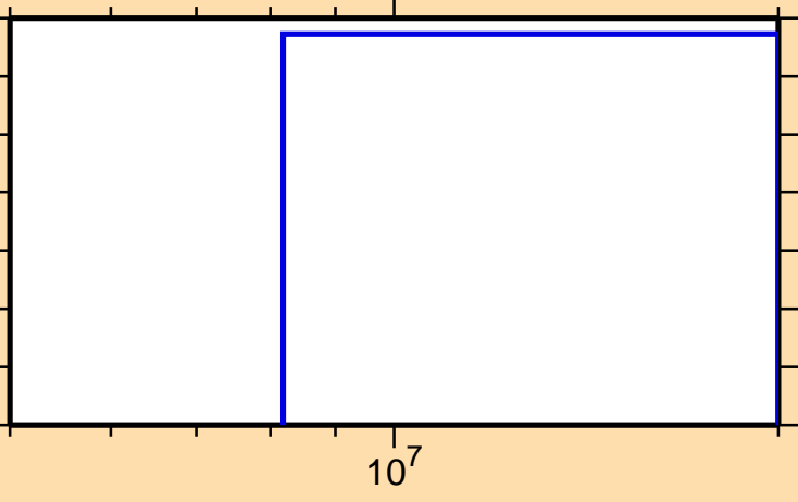
\sigma vs. E for ^{155}\text{Nd}(n,n\alpha)
