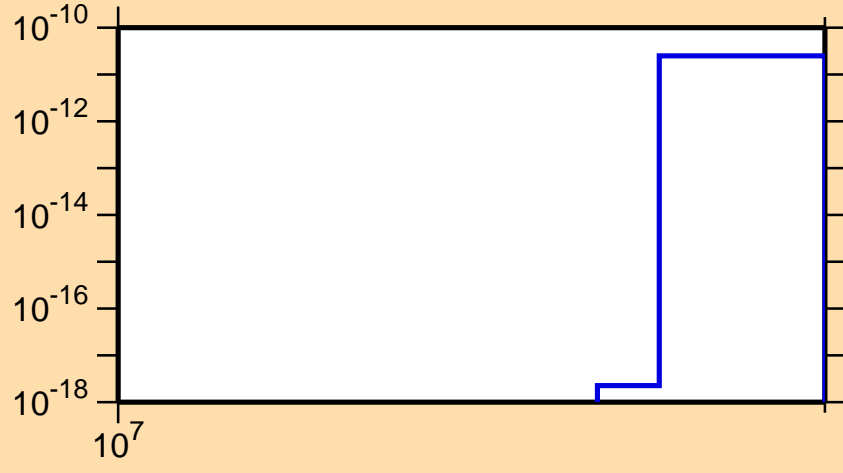
\sigma vs. E for ^{157}\text{Nd}(n,2np)
