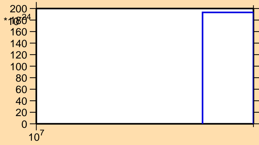
\sigma vs. E for ^{157}\text{Nd} (mt 11)
