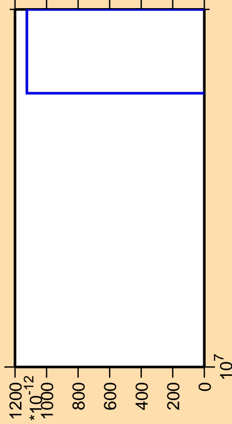
\Delta\sigma/\sigma vs. E for ^{157}\text{Nd} (mt 11)
