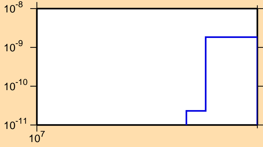
\sigma vs. E for ^{157}\text{Nd}(n,2n\alpha)
