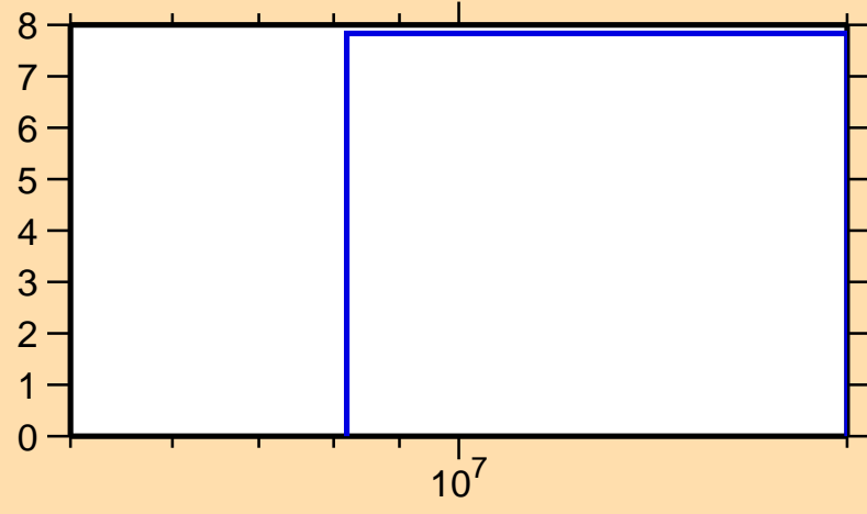
\Delta\sigma/\sigma vs. E for ^{157}\text{Nd}(n,\text{nonel.})
