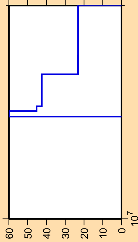
\Delta\sigma/\sigma vs. E for ^{19}\text{Ne}(n,nd)
