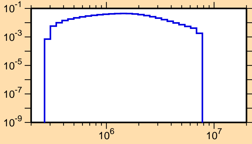
\sigma vs. E for ^{19}\text{Ne}(n,n_2)
