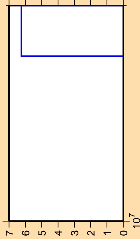
\Delta\sigma/\sigma vs. E for ^{19}\text{Ne}(n,2n\alpha)
