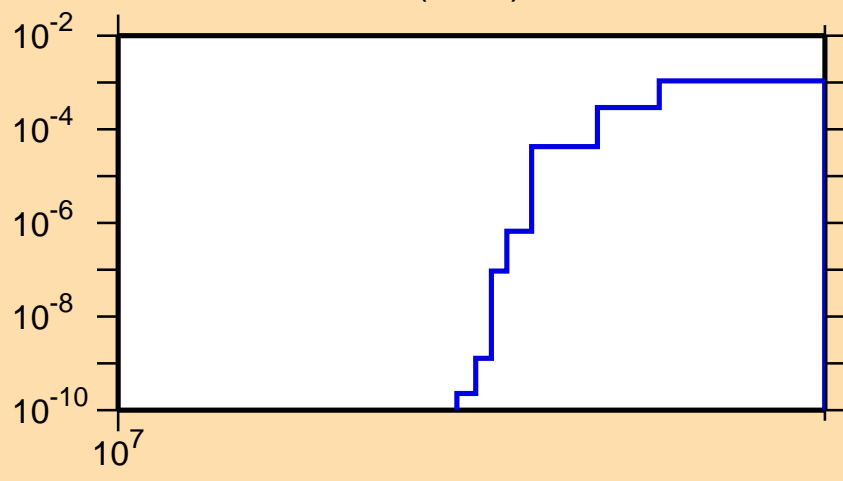
\sigma vs. E for ^{19}\text{Ne}(n,nd)
