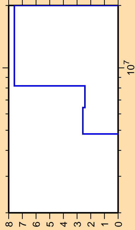
\Delta\sigma/\sigma vs. E for ^{20}\text{Ne}(n,n_4)
