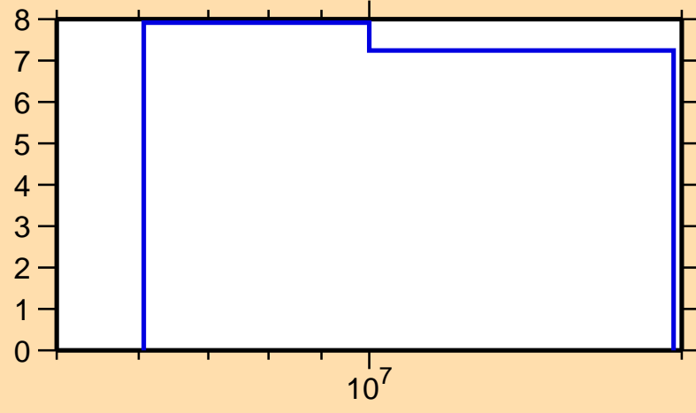
\Delta\sigma/\sigma vs. E for ^{21}\text{Ne}(n,2n)
