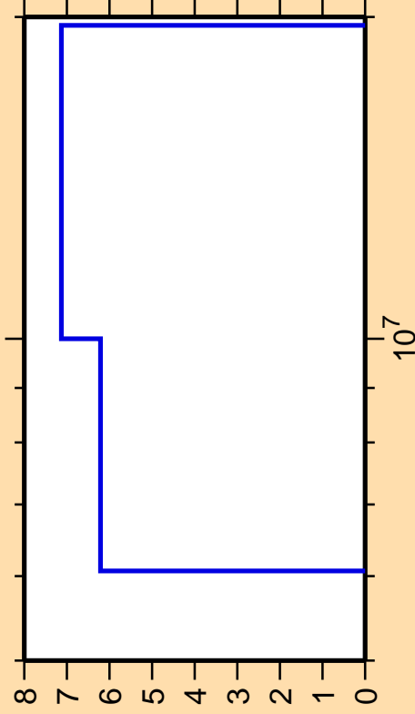
\Delta\sigma/\sigma vs. E for ^{21}\text{Ne}(n,n\alpha)
