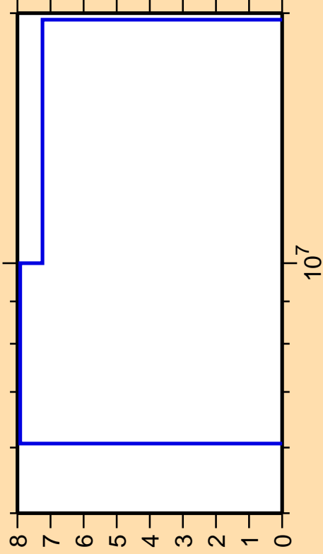
\Delta\sigma/\sigma vs. E for ^{21}\text{Ne}(n,2n)
