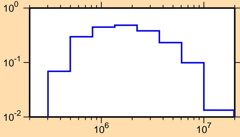
\sigma vs. E for ^{21}\text{Ne}(n,n_1)
