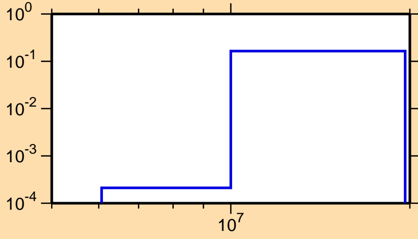
\sigma vs. E for ^{21}\text{Ne}(n,n\alpha)
