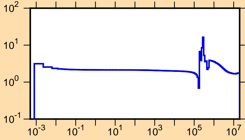
\sigma vs. E for ^{22}\text{Ne}(n,\text{tot.})
