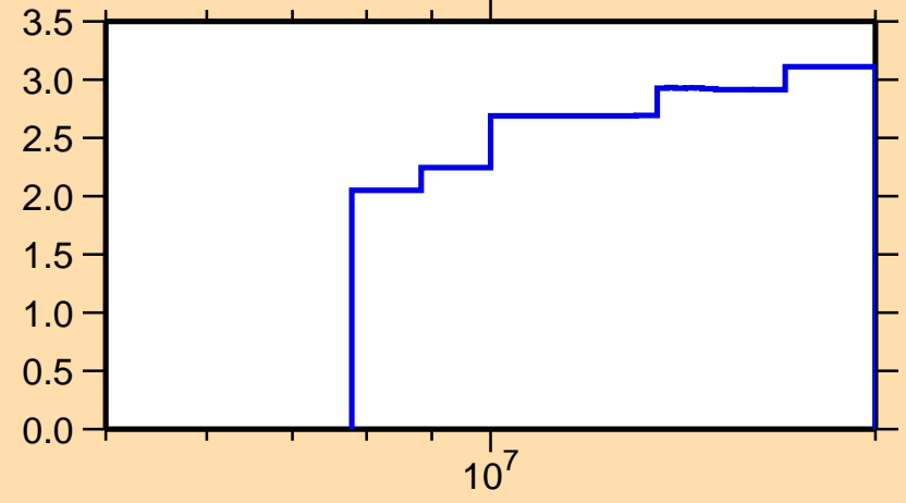
\Delta\sigma/\sigma vs. E for ^{22}\text{Ne}(n,\text{nonel.})
