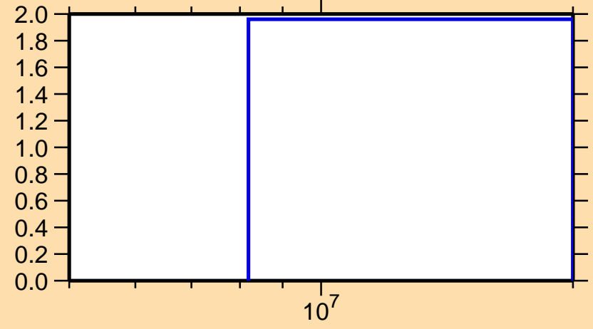
\Delta\sigma/\sigma vs. E for ^{22}\text{Ne}(n,\text{inel.})
