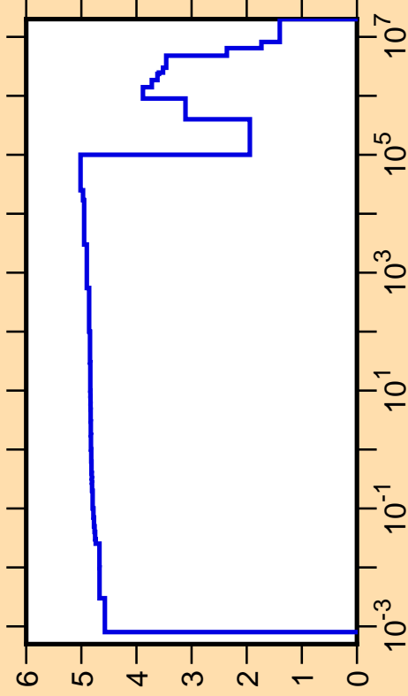
\Delta\sigma/\sigma vs. E for ^{22}\text{Ne}(n,\text{tot.})
