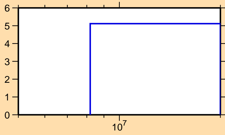
\Delta\sigma/\sigma vs. E for ^{22}\text{Ne}(n,2n)
