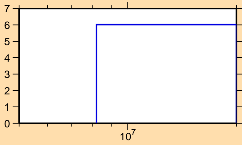
\Delta\sigma/\sigma vs. E for ^{22}\text{Ne}(n,n\text{cont.})
