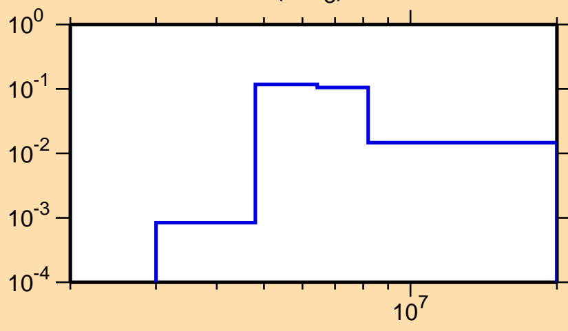
\sigma vs. E for ^{22}\text{Ne}(n,n_3)
