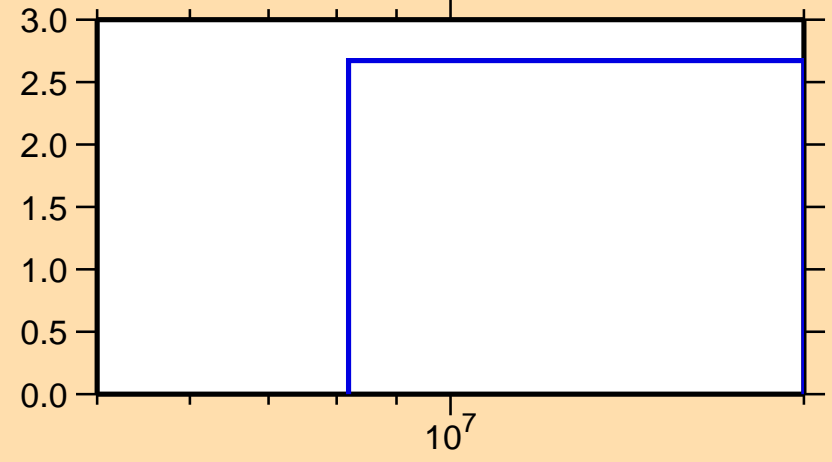
\Delta\sigma/\sigma vs. E for ^{22}\text{Ne}(n,n\text{onel.})
