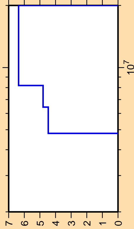
\Delta\sigma/\sigma vs. E for ^{22}\text{Ne}(n,n_4)
