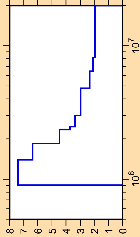
\Delta\sigma/\sigma vs. E for ^{22}\text{Ne}(n,\text{inel.})
