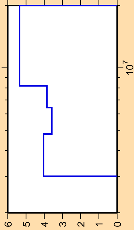
\Delta\sigma/\sigma vs. E for ^{22}\text{Ne}(n,n_3)
