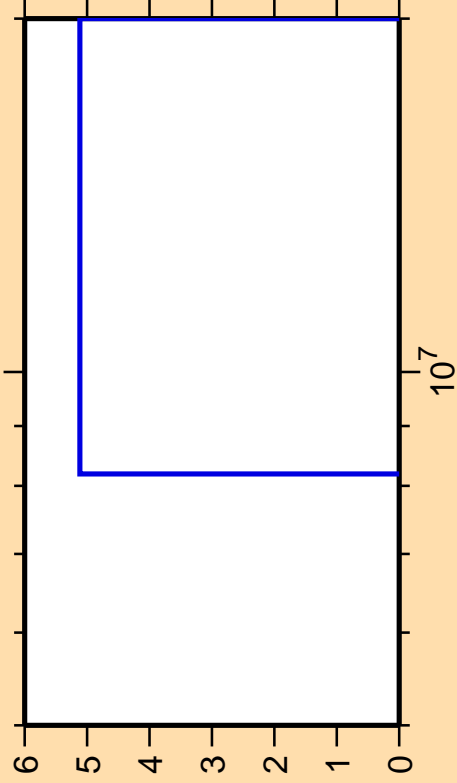
\Delta\sigma/\sigma vs. E for ^{22}\text{Ne}(n,2n)
