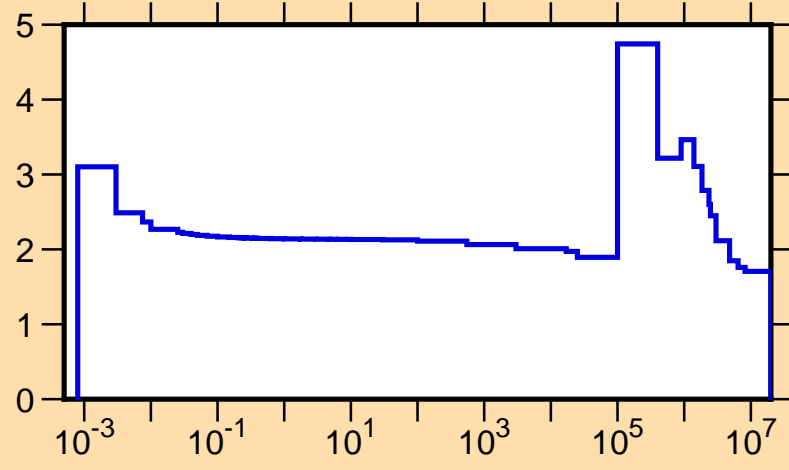
\sigma vs. E for ^{22}\text{Ne}(n,\text{tot.})
