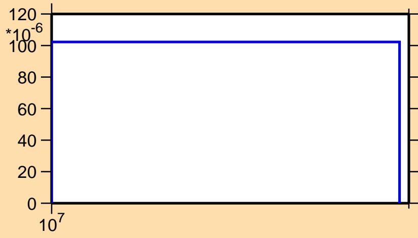
\sigma vs. E for ^{23}\text{Ne}(n,d)
