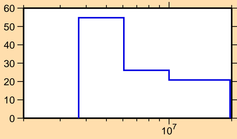
\Delta\sigma/\sigma vs. E for ^{23}\text{Ne}(n,n\text{cont.})
