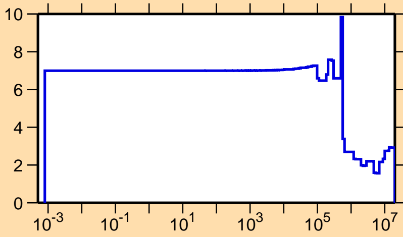
\Delta\sigma/\sigma vs. E for ^{24}\text{Ne}(n,\text{el.})
