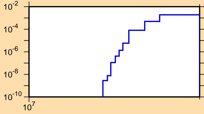
\sigma vs. E for ^{24}\text{Ne}(n,n\alpha)
