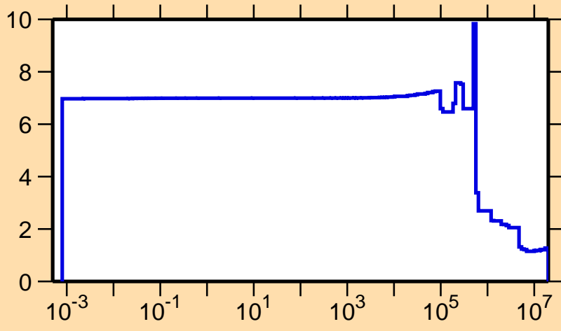
\Delta\sigma/\sigma vs. E for ^{24}\text{Ne}(n,\text{tot.})
