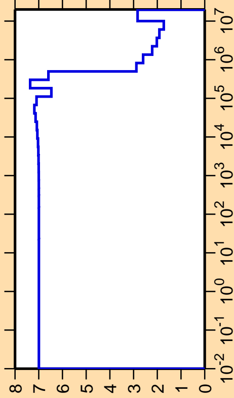
\Delta\sigma/\sigma vs. E for ^{24}\text{Ne}(n,\text{el.})
