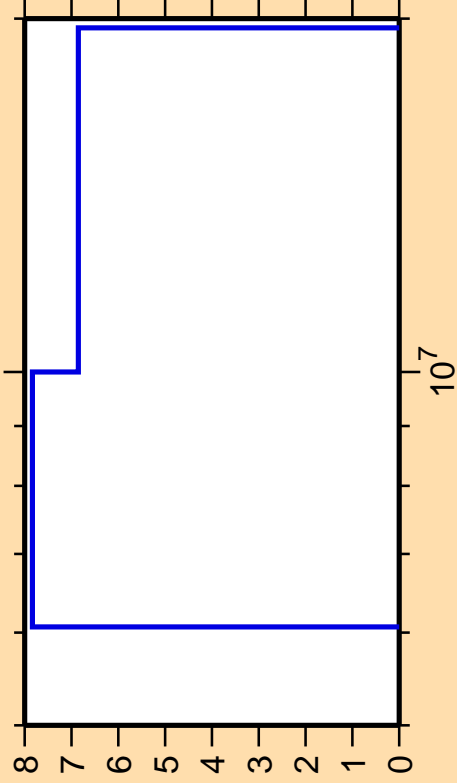
\Delta\sigma/\sigma vs. E for ^{24}\text{Ne}(n,\alpha)
