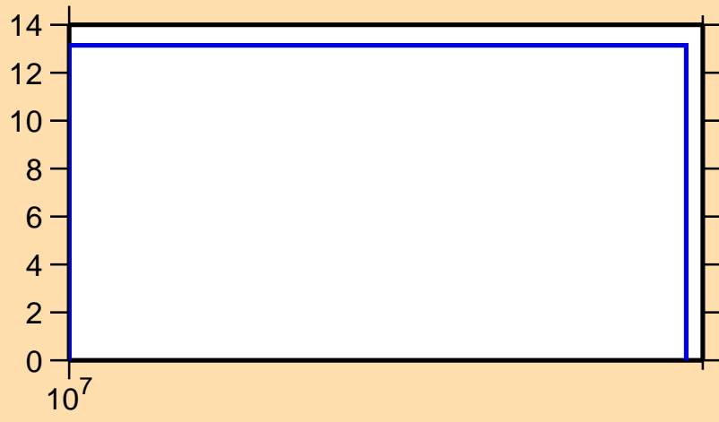
\Delta\sigma/\sigma vs. E for ^{24}\text{Ne}(n,p)
