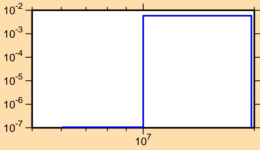
\sigma vs. E for ^{24}\text{Ne}(n,\alpha)
