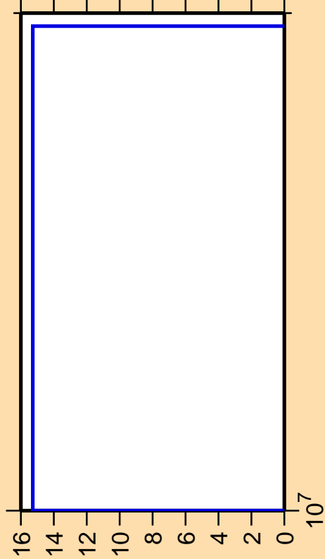
\Delta\sigma/\sigma vs. E for ^{24}\text{Ne}(n,\text{ncont.})
