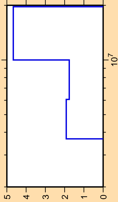
\Delta\sigma/\sigma vs. E for ^{24}\text{Ne}(n,n_3)
