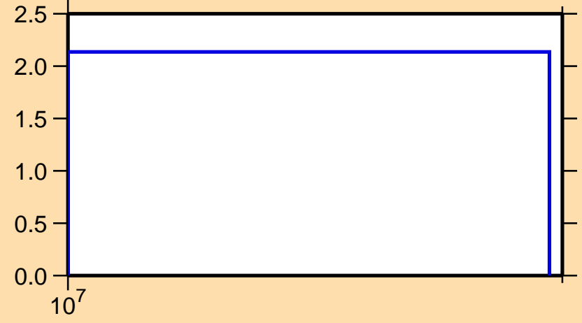
\Delta\sigma/\sigma vs. E for ^{24}\text{Ne}(n,n\text{nonel.})
