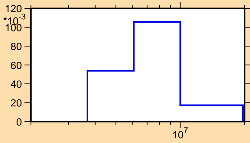
\sigma vs. E for ^{24}\text{Ne}(n,n_3)
