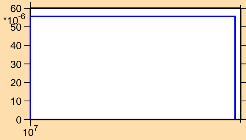
\sigma vs. E for ^{24}\text{Ne}(n,n\alpha)
