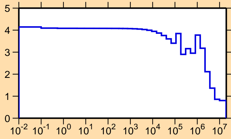
\sigma vs. E for ^{24}\text{Ne}(n,\text{el.})
