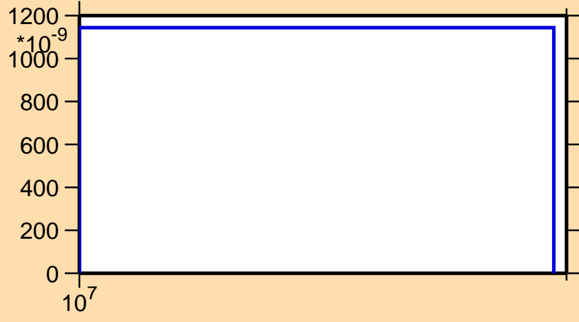
\sigma vs. E for ^{24}\text{Ne}(n,t)
