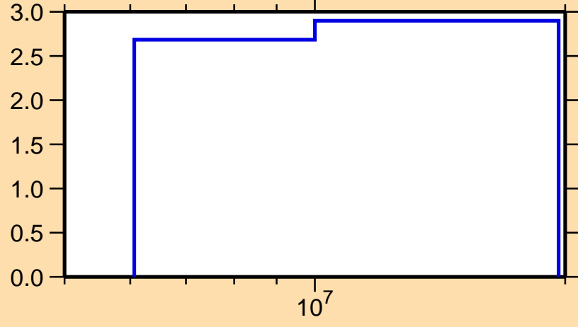
\Delta\sigma/\sigma vs. E for ^{24}\text{Ne}(n,2n)
