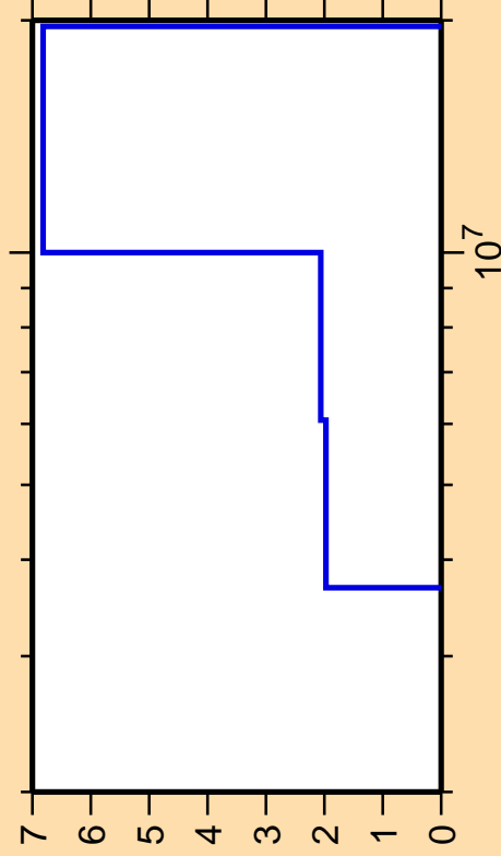
\Delta\sigma/\sigma vs. E for ^{24}\text{Ne}(n,n_2)
