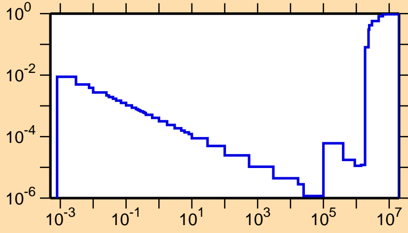
\sigma vs. E for ^{24}\text{Ne}(n,\text{nonel.})
