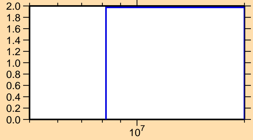
\Delta\sigma/\sigma vs. E for ^{24}\text{Ne}(n,\text{inel.})
