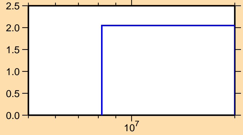
\Delta\sigma/\sigma vs. E for ^{24}\text{Ne}(n,n\text{onel.})
