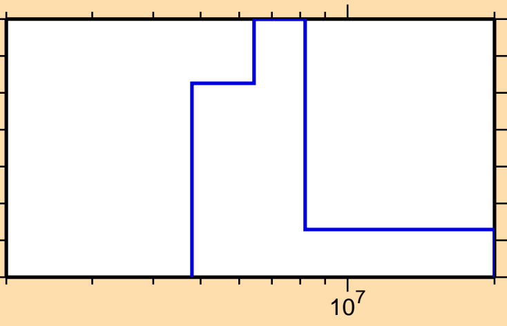
\sigma vs. E for ^{24}\text{Ne}(n,n_4)
