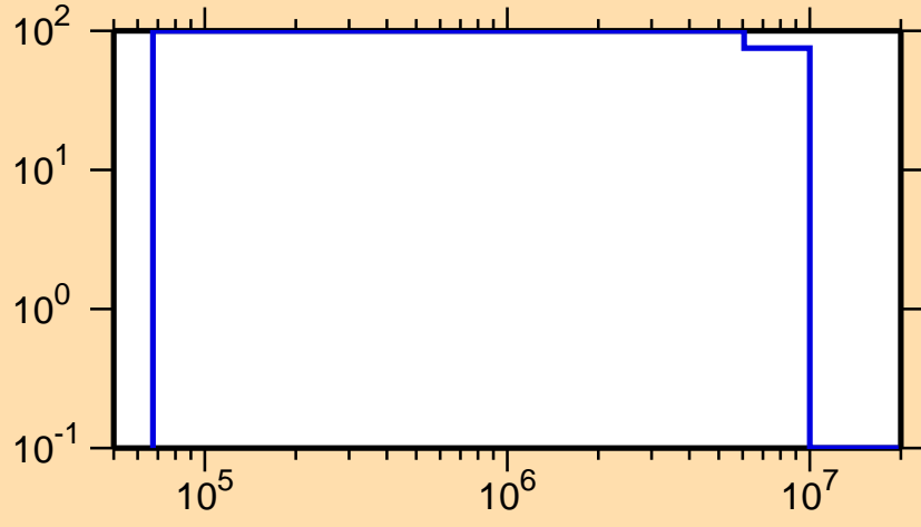
\Delta\sigma/\sigma vs. E for ^{284}_1
