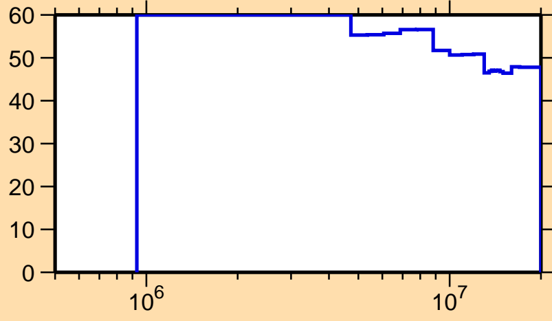
\Delta\sigma/\sigma vs. E for ^{285}_{1}
