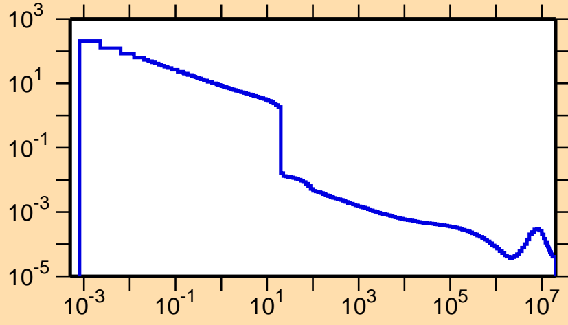
\sigma vs. E for ^{285}\gamma
