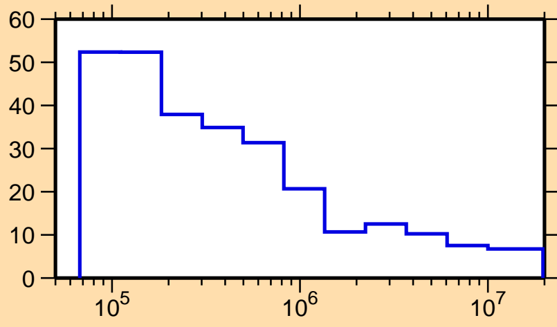
\Delta\sigma/\sigma vs. E for ^{285}\text{Po}
