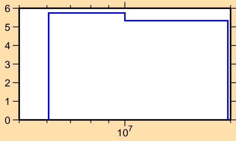
\Delta\sigma/\sigma vs. E for ^{287}\text{Fr}
