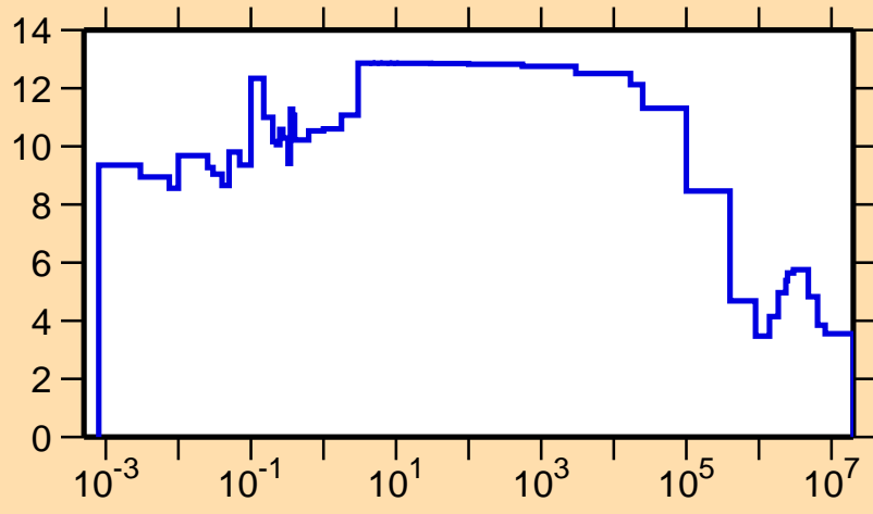
\sigma vs. E for ^{287}
