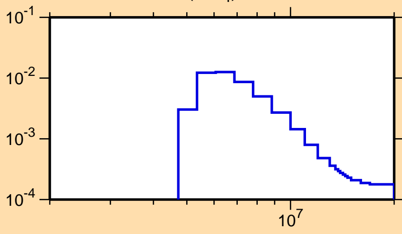
\sigma vs. E for ^{56}\text{Ni}(n,n_4)
