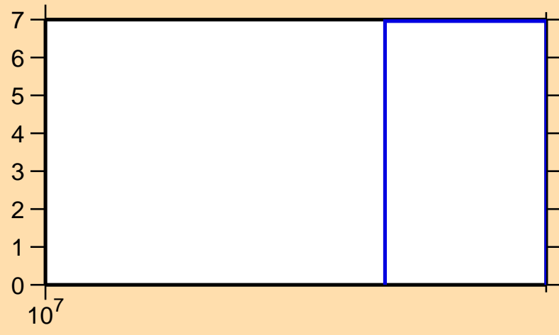
\Delta\sigma/\sigma vs. E for ^{56}\text{Ni}(n,\text{inel.})
