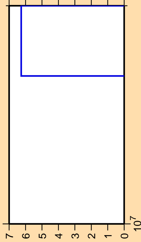
\Delta\sigma/\sigma vs. E for ^{56}\text{Ni}(n,n_1)
