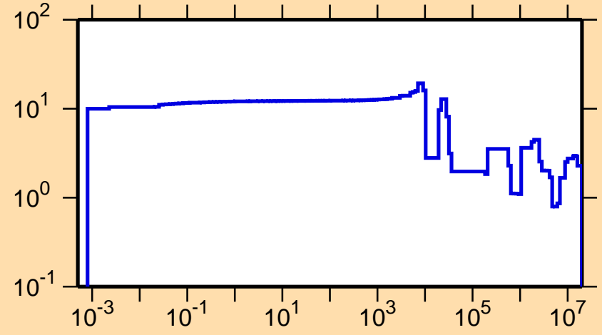
\Delta\sigma/\sigma vs. E for ^{56}\text{Ni}(n,\text{tot.})
