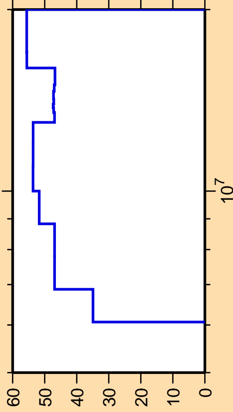
\Delta\sigma/\sigma vs. E for ^{56}\text{Ni}(n,\alpha)
