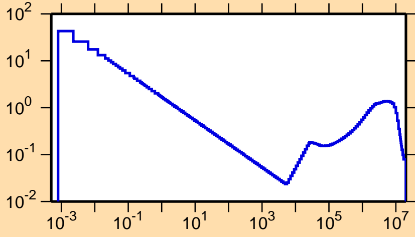
\sigma vs. E for ^{56}\text{Ni}(n,p)
