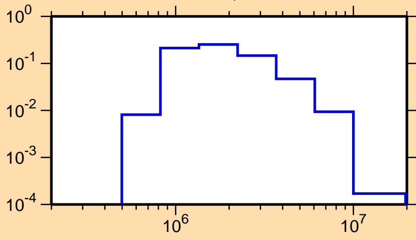
\sigma vs. E for ^{57}\text{Ni}(n,n_1)
