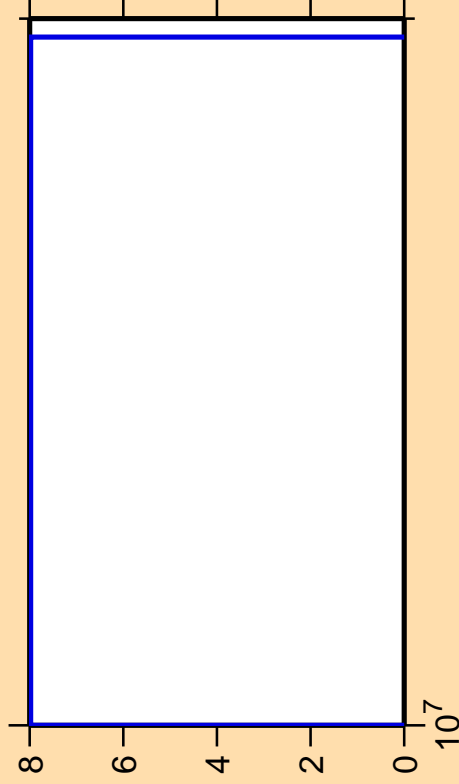
\Delta\sigma/\sigma vs. E for ^{57}\text{Ni} (mt 34)
