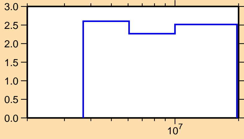
\Delta\sigma/\sigma vs. E for ^{57}\text{Ni}(n,n\text{onel.})
