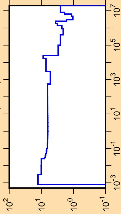
\Delta\sigma/\sigma vs. E for ^{57}\text{Ni}(n,\text{tot.})
