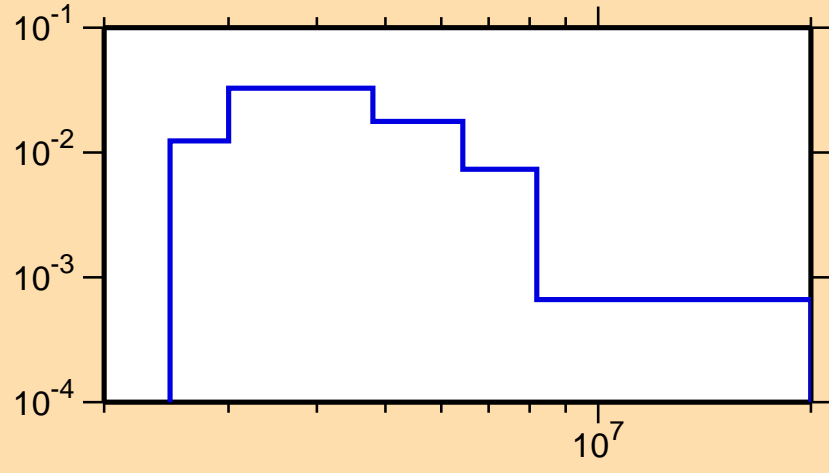
\sigma vs. E for ^{57}\text{Ni}(n,n_4)
