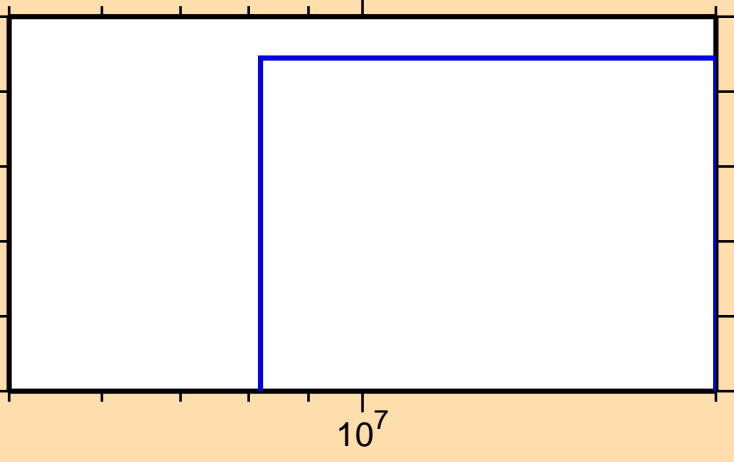
\sigma vs. E for ^{57}\text{Ni}(n,\text{nd})
