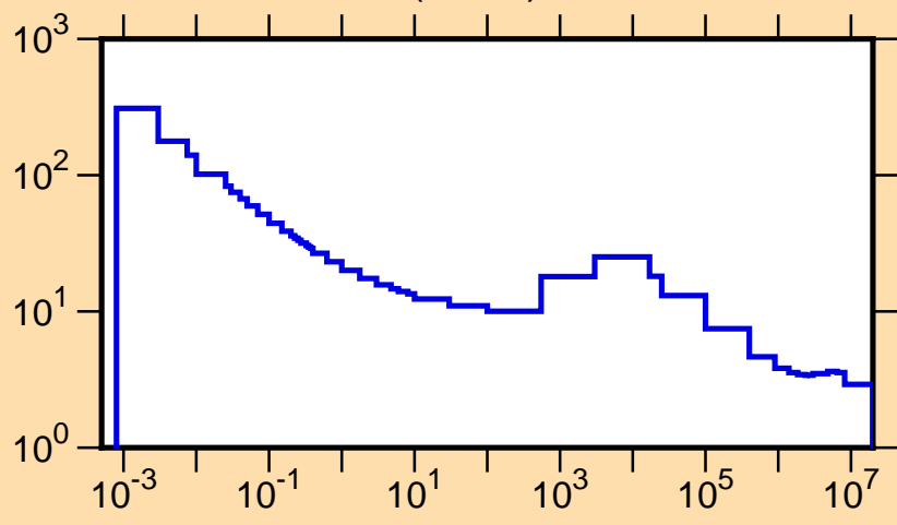
\sigma vs. E for ^{57}\text{Ni}(n,\text{tot.})
