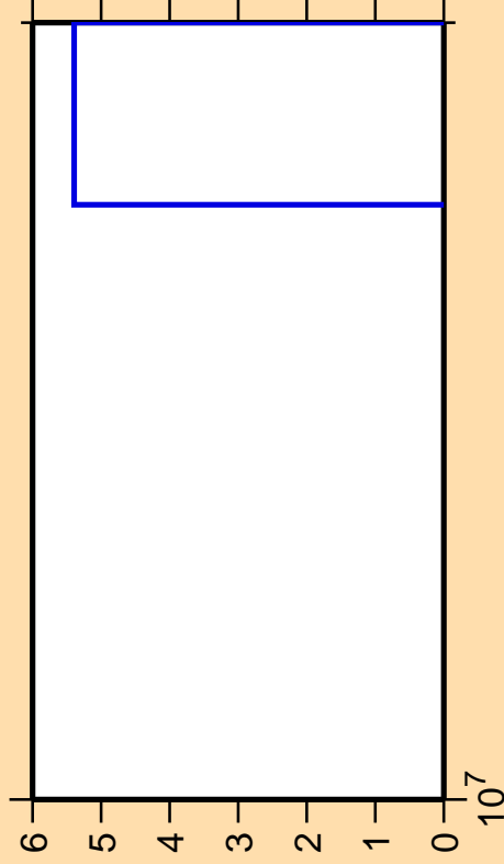
\Delta\sigma/\sigma vs. E for ^{58}\text{Ni}(n,2np)
