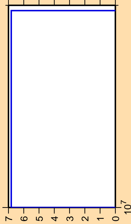
\Delta\sigma/\sigma vs. E for ^{58}\text{Ni}(n,p)
