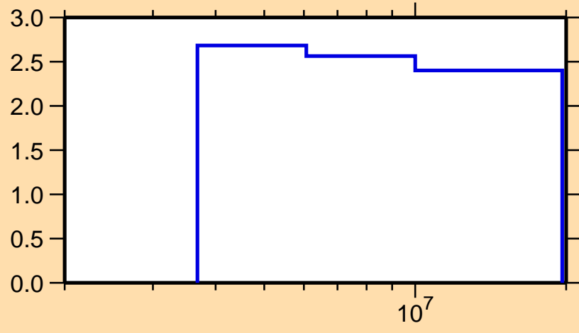
\Delta\sigma/\sigma vs. E for ^{58}\text{Ni}(n,n\text{onel.})
