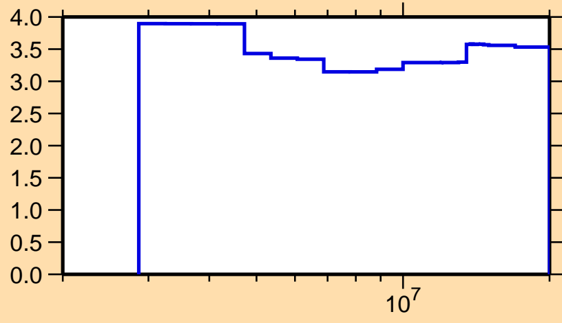
\Delta\sigma/\sigma vs. E for ^{59}\text{Ni}(n,n\text{nonel.})
