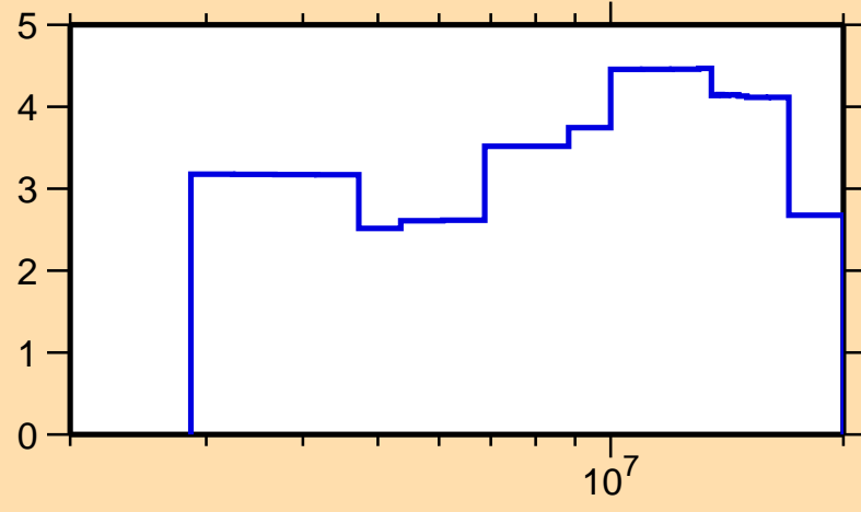
\Delta\sigma/\sigma vs. E for ^{59}\text{Ni}(n, el.)
