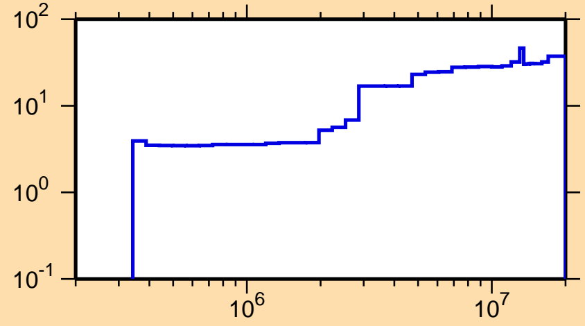
\Delta\sigma/\sigma vs. E for ^{59}\text{Ni}(n,n_1)
