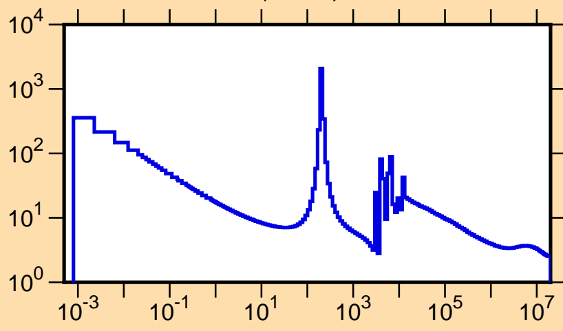
\sigma vs. E for ^{59}\text{Ni}(n,\text{tot.})
