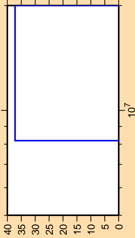
\Delta\sigma/\sigma vs. E for ^{59}\text{Ni}(n,\alpha)
