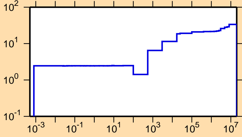
\Delta\sigma/\sigma vs. E for ^{59}\text{Ni}(n,\gamma)
