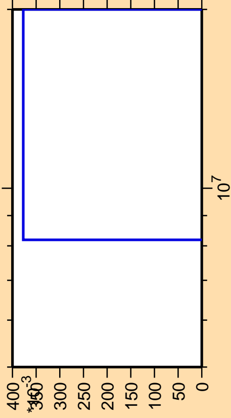
\Delta\sigma/\sigma vs. E for ^{59}\text{Ni} (mt 34)
