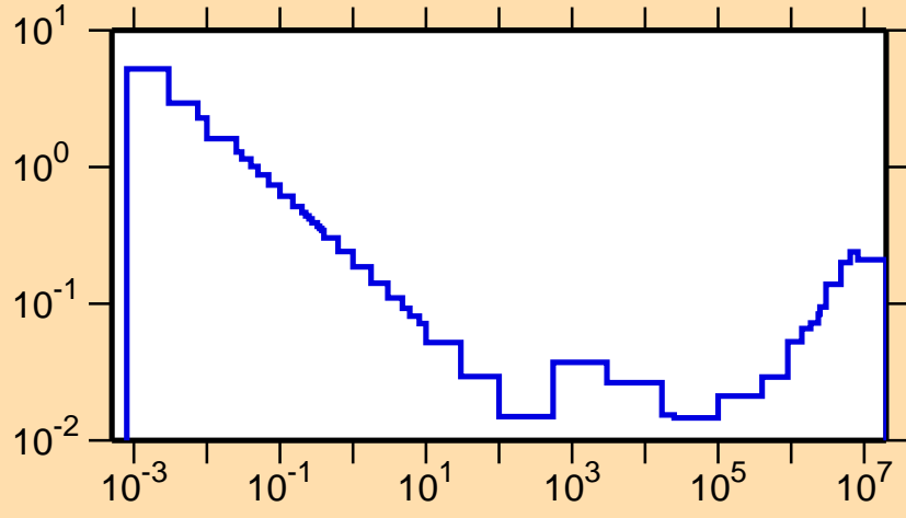
\sigma vs. E for ^{59}\text{Ni}(n,p)
