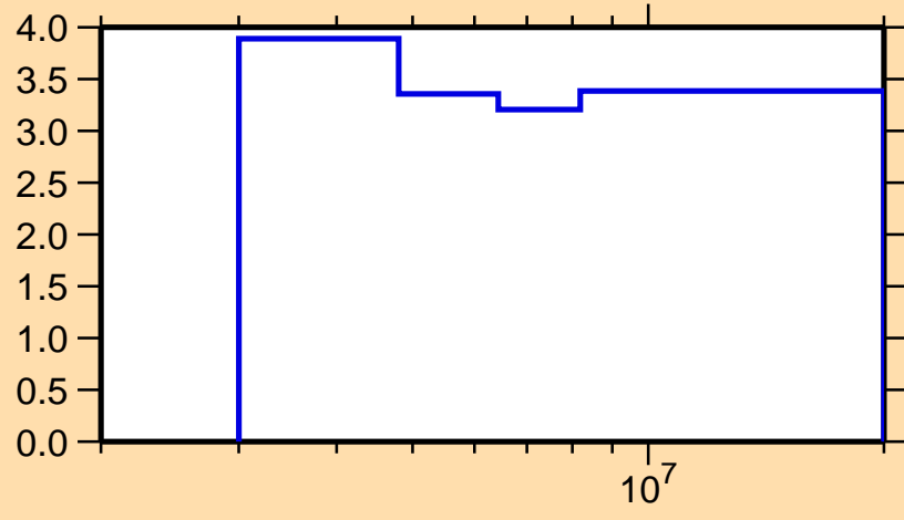
\Delta\sigma/\sigma vs. E for ^{59}\text{Ni}(n,n\text{onel.})
