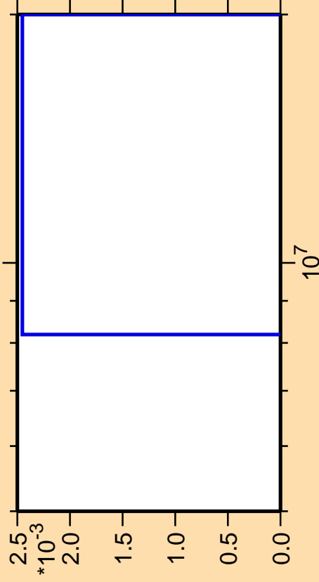
\Delta\sigma/\sigma vs. E for ^{59}\text{Ni}(\text{mt117})
