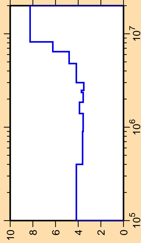
\Delta\sigma/\sigma vs. E for ^{59}\text{Ni}(n,\text{inel.})
