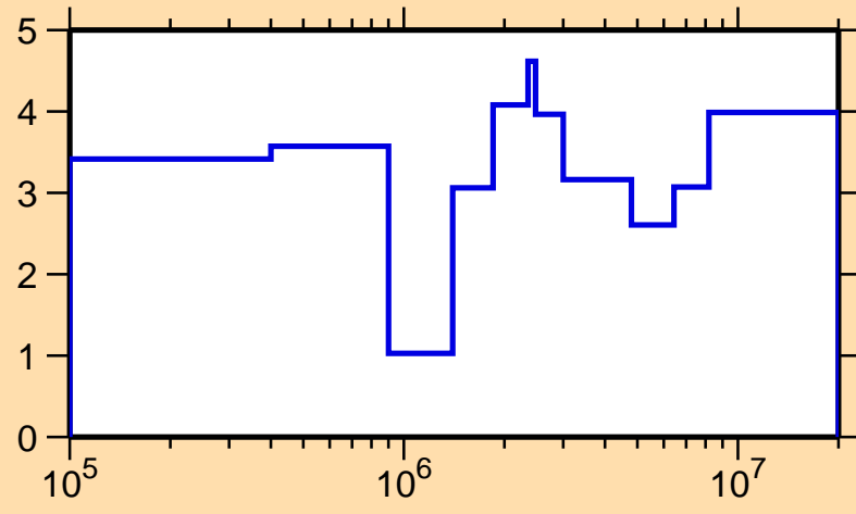
\Delta\sigma/\sigma vs. E for ^{59}\text{Ni}(n,\text{el.})
